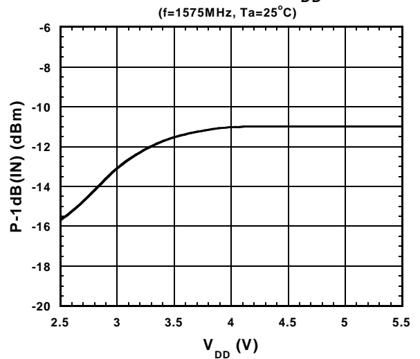
P-1dB(IN) vs. V_{DD}
