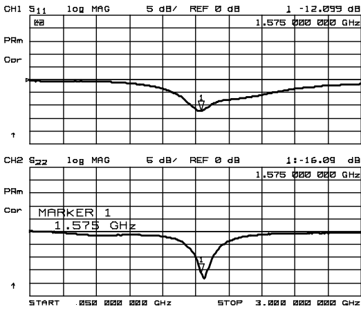
S 11 , S 22
