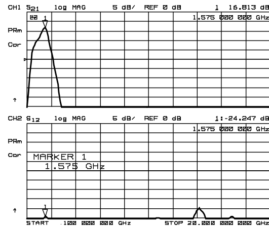
S 21 , S 12 (~20GHz)
