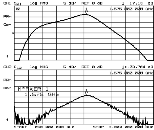
S 21 , S 12
