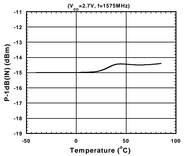
P-1dB(IN) vs. Temperature
