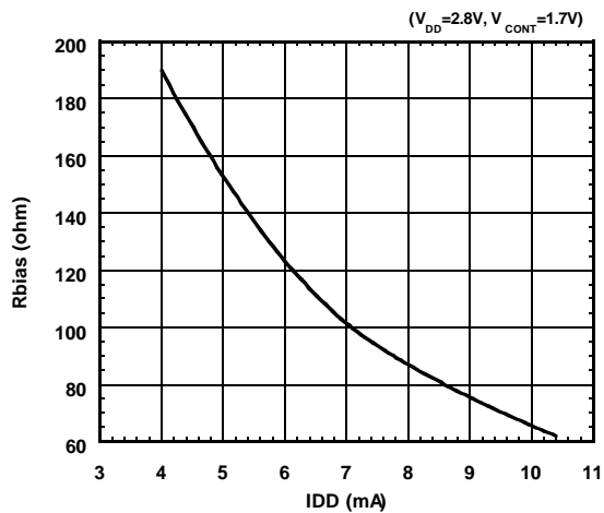
Rbias vs. IDD
