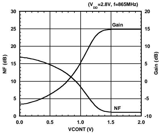
NF,Gain vs. VCONT
