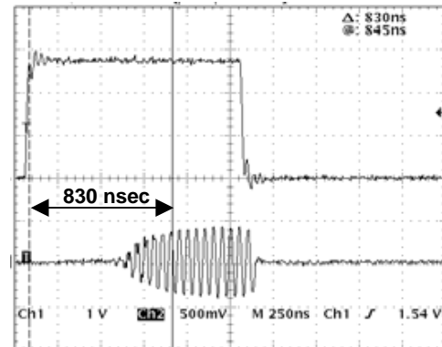
Switching Speed ( Vctl(L)=0V, Vctl(H)=2.7V )
