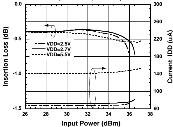
Insertion Loss, Current IDD vs. Input Power
