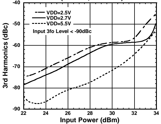
3rd Harmonics vs.Input Power
