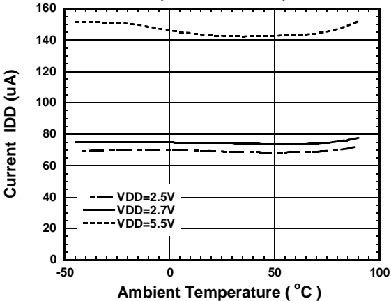
Current IDD vs. Ambient Temperature
