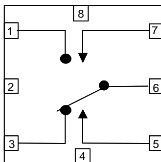
USB8-B3 Type (TOP VIEW)
