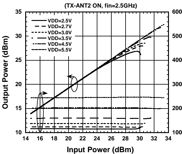
Output Power, IDD vs. Input Power
