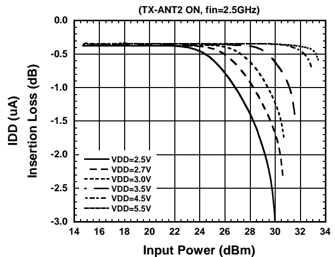
Insertion Loss vs. Input Power
