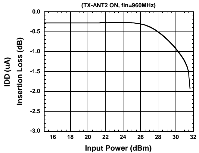
Insertion Loss vs. Input Power
