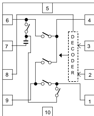
USB10-C3 Type (TOP VIEW)
