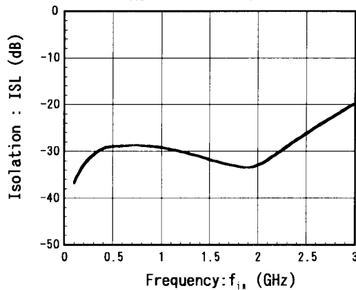
(PC-P2) Isolation vs. Frequency ( V_{CT1}=0V/2.7V , P_{i1}=0dBm )
