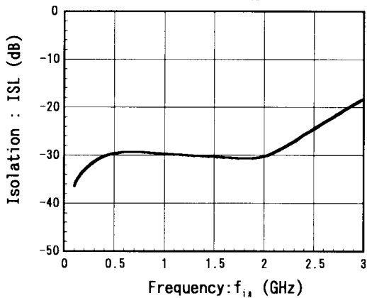
(PC-P1) Isolation vs. Frequency ( V_{CT1}=0V/2.7V , P_{i1}=0dBm )
