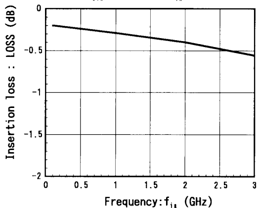
(PC-P1) Insertion loss vs. Frequency ( V_{CT1}=0V/2.7V , P_{i1}=0dBm )
