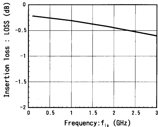
(PC-P2) Insertion loss vs. Frequency ( V_{CT1}=0V/2.7V , P_{i1}=0dBm )
