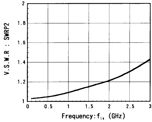
P2-PC(ON) V.S.W.R vs. Frequency
