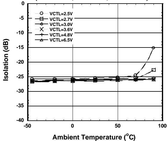
PC-P3 Isolation vs. Ambient Temperature
