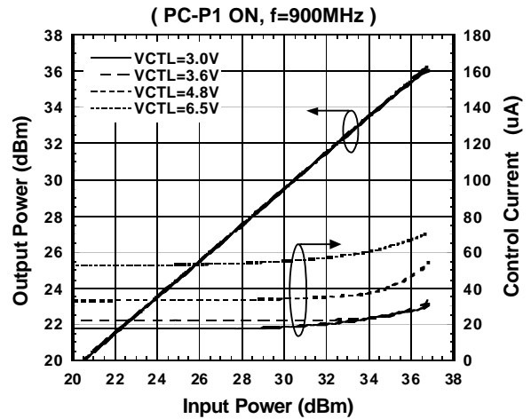
Output Power,Control Current vs. Input Power
