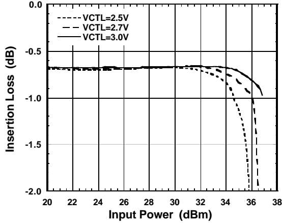
Insertion Loss vs. Input Power ( PC-P1 ON, f=1.9GHz )
