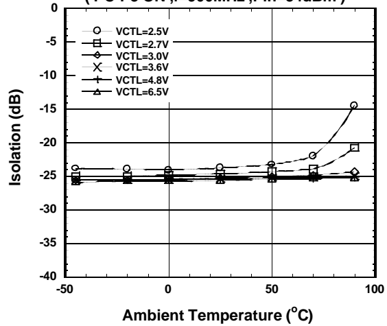
PC-P2 Isolation vs. Ambient Temperature
