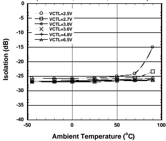
PC-P1 Isolation vs. Ambient Temperature
