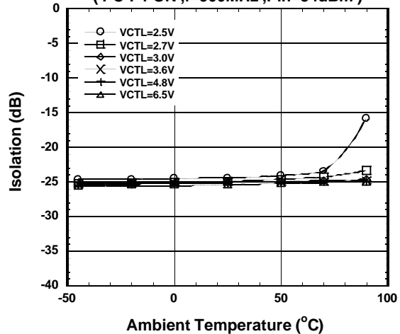
PC-P4 Isolation vs. Ambient Temperature
