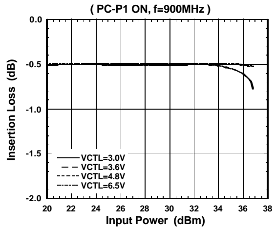
Insertion Loss vs. Input Power
