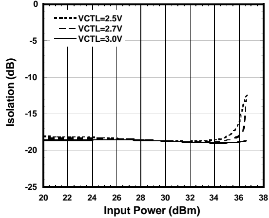
PC-P1 Isolation vs. Input Power ( PC-P4 ON, f=1.9GHz )
