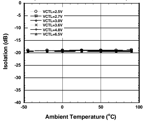
PC-P2 Isolation vs. Ambient Temperature ( PC-P3 ON ,f=1.9GHz ,Pin=32dBm )
