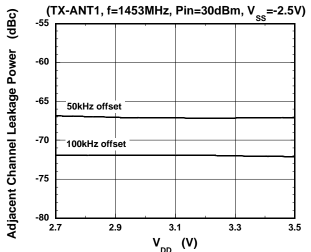
ACP vs. V_{DD}
