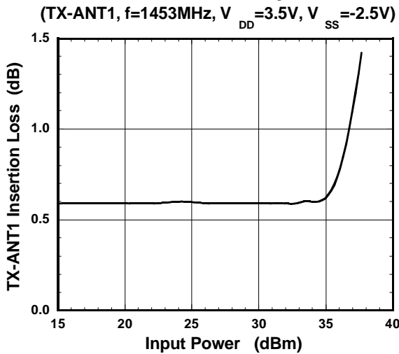
Insertion Loss vs. Input Power
