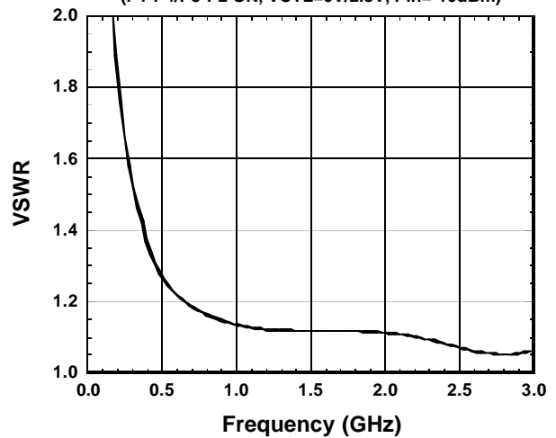
P3-P2 VSWR vs. Frequency
