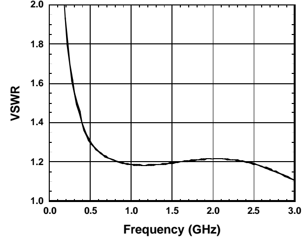
P3-P4 VSWR vs. Frequency
