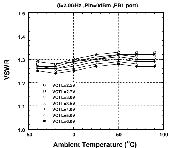
PC2-PB1(on) VSWR vs. Ambient Temperature
