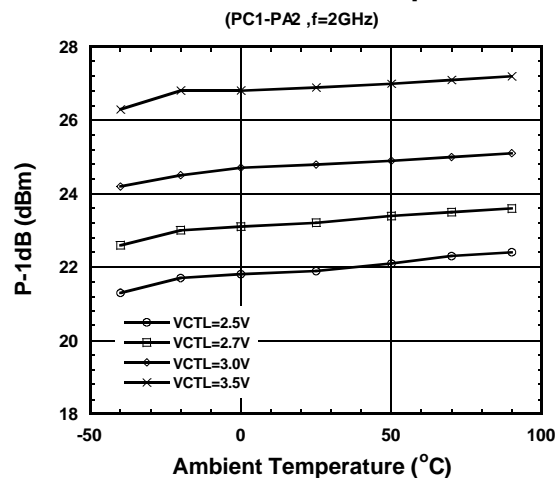
P-1dB vs. Ambient Temperature
