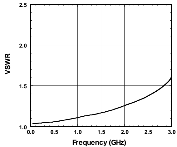
PC1-PA1(on) VSWR vs. Frequency
