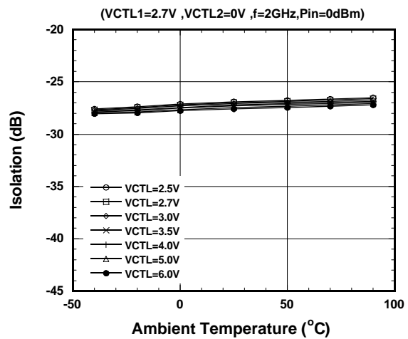
PA1-PA2 Isolation vs. Ambient Temperature
