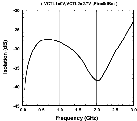
PC1-PA1 Isolation vs. Frequency
