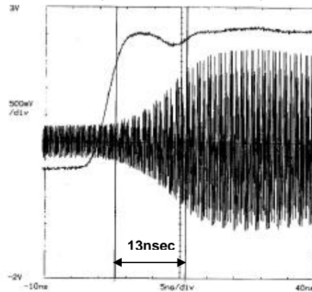
Switching Speed (VCTL=2.7V,Pin=10dBm)
