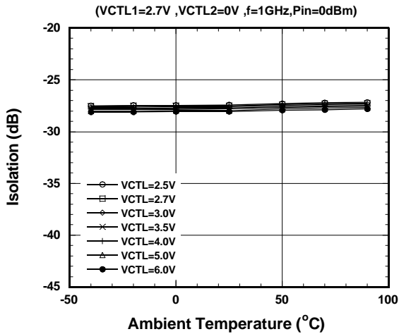
PA1-PA2 Isolation vs. Ambient Temperature
