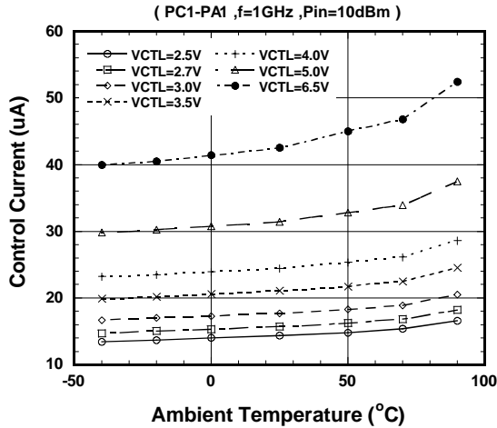
Control Current vs. Ambient Temperature
