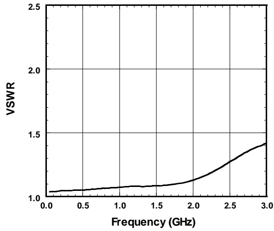
PC1-PA2(on) VSWR vs. Frequency
