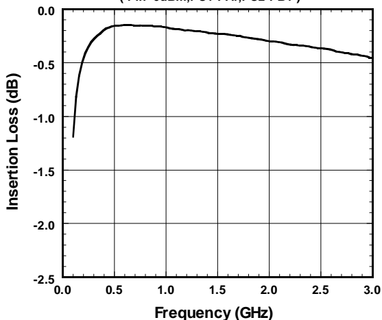
PCB Through Loss vs. Frequency
