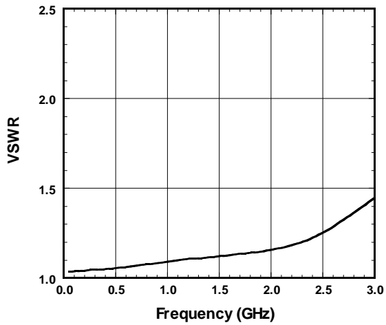
PC2-PB2(on) VSWR vs. Frequency
