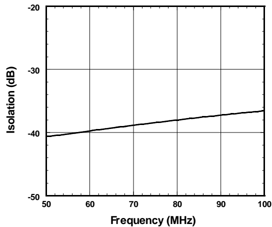
PC1-PC2 Isolation vs. Frequency
