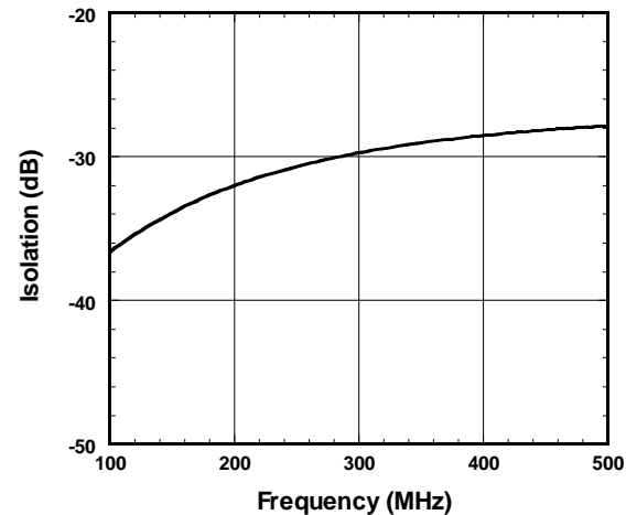
PB1-PB2 Isolation vs. Frequency
