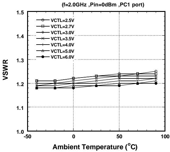
PC1-PA2(on) VSWR vs. Ambient Temperature
