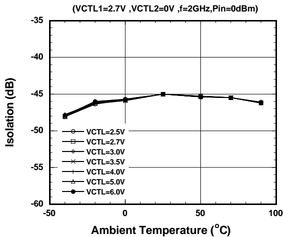
PC1-PC2 Isolation vs. Ambient Temperature
