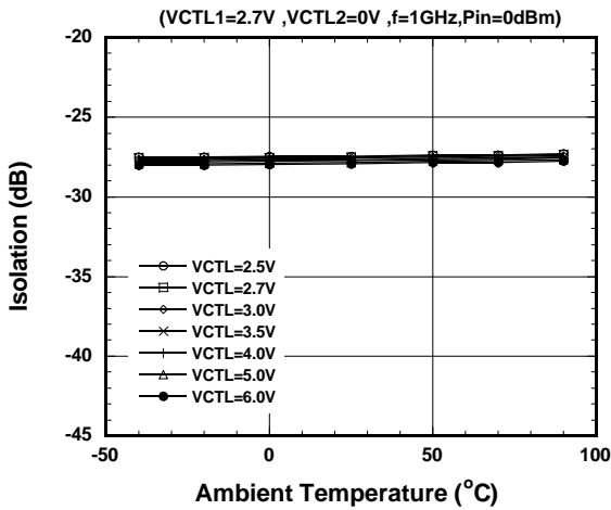
PC1-PA2 Isolation vs. Ambient Temperature
