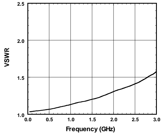
PC2-PB1(on) VSWR vs. Frequency
