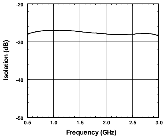
PB1-PB2 Isolation vs. Frequency
