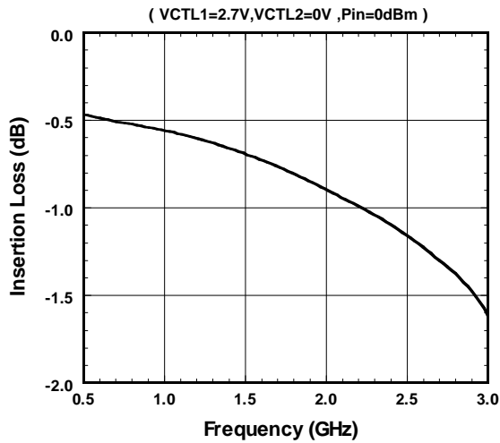
PC2-PB1 Insertion Loss vs. Frequency
