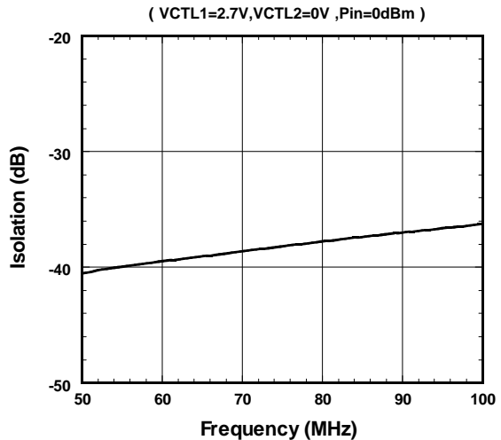
PC1-PA2 Isolation vs. Frequency
