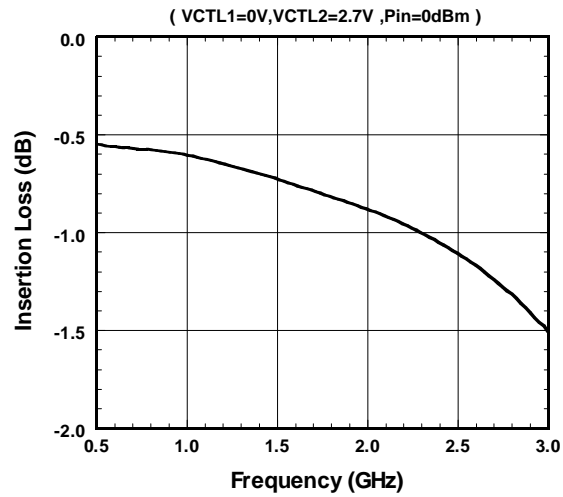
PC2-PB2 Insertion Loss vs. Frequency
