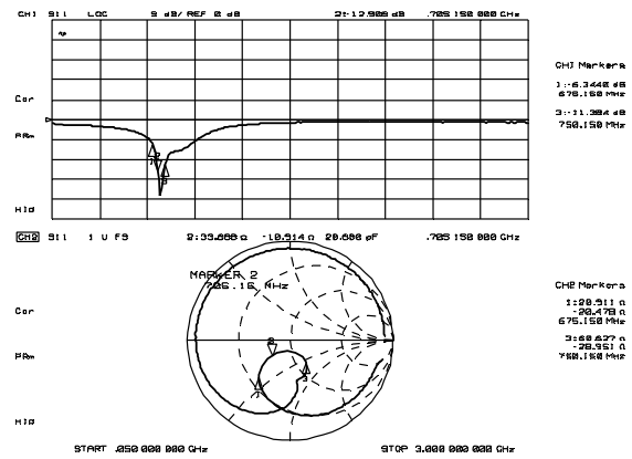
LOCAL IN Port Impedance (MIXER IN Port, IF OUT Port: 50 ohm term.)
