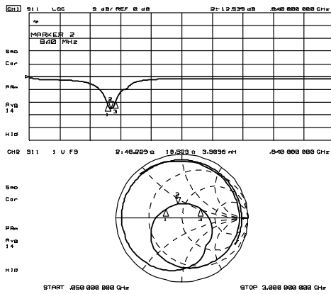
MIXER IN Port Impedance ( P_{LO} = -15\text{dBm} , IF OUT Port: 50ohm term.)
