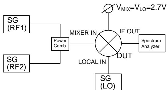
IF,IM3 Measurement Block Diagram
