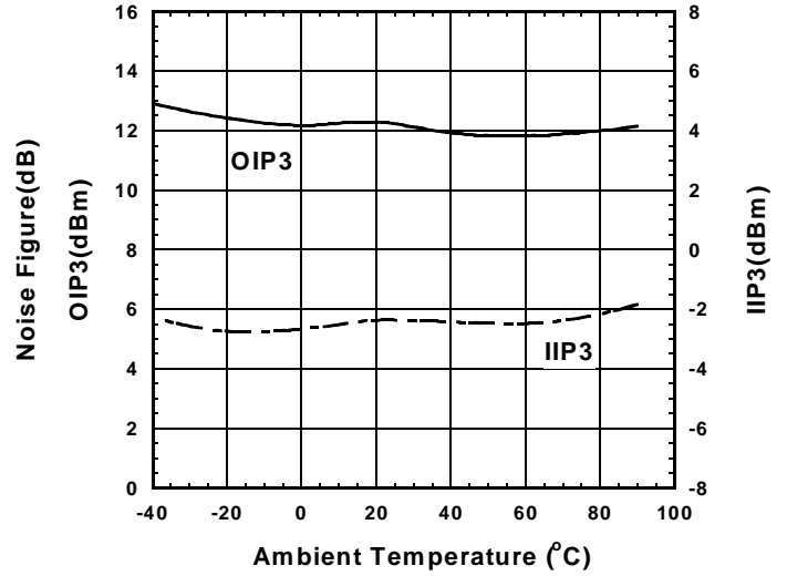
OIP3, IIP3 vs. Temperature
