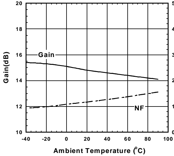
Gain, Noise Figure vs. Temperature
