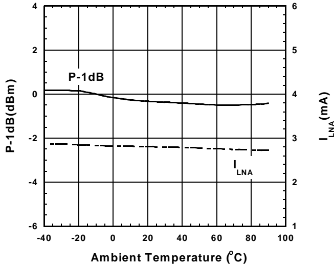
P-1dB, I_{LNA} vs. Temperature
