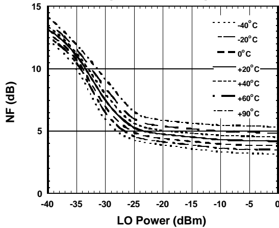
Noise Figure vs. Local Power Temperature Response
