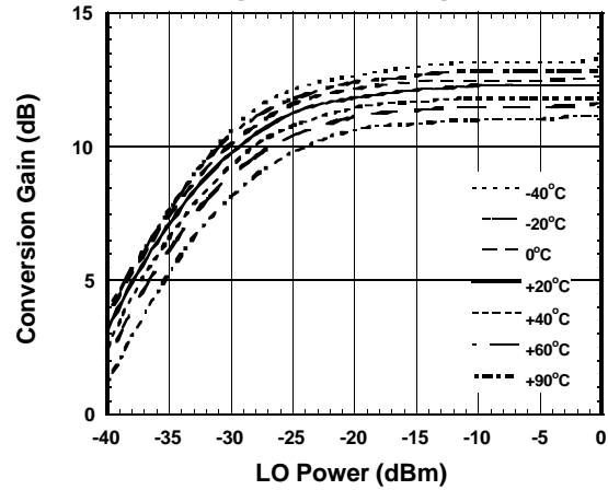
Conversion Gain vs. Local Power Temperature Response
