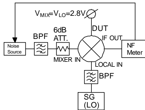
Noise Figure Measuring Block Diagram
