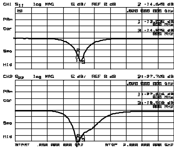
S11, S22
