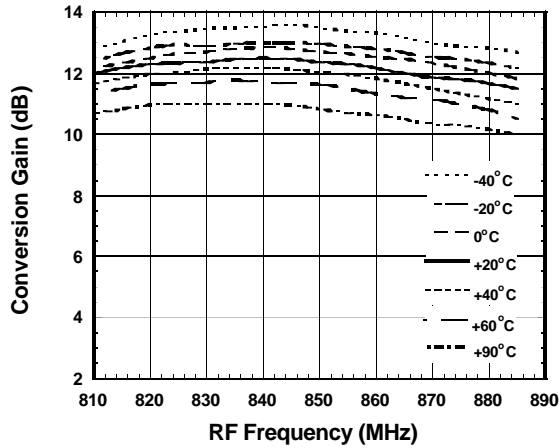
Conversion Gain vs. RF Frequency Temperature Response
