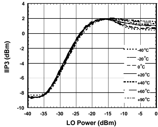
IIP3 vs. Local Power Temperature Response
