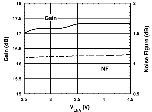
Gain, NF vs. V_{LNA}
