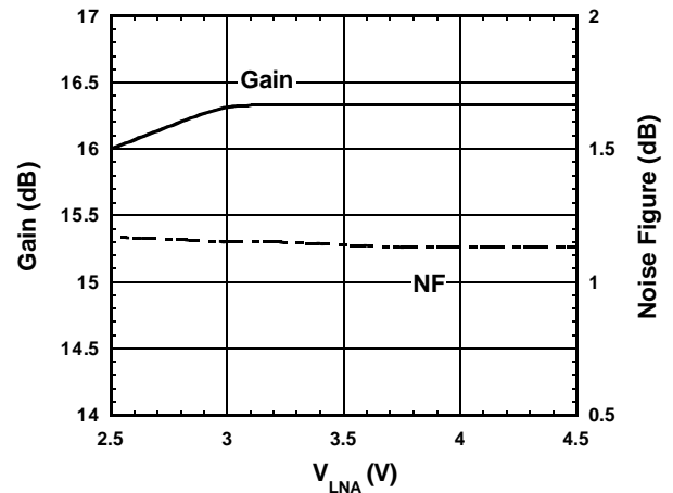
Gain, NF vs. V_{LNA} ( f=1900\text{MHz} )
