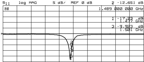
MIXER IN PORT IMPEDANCE ( P_{LO}=-15\text{dBm} )
