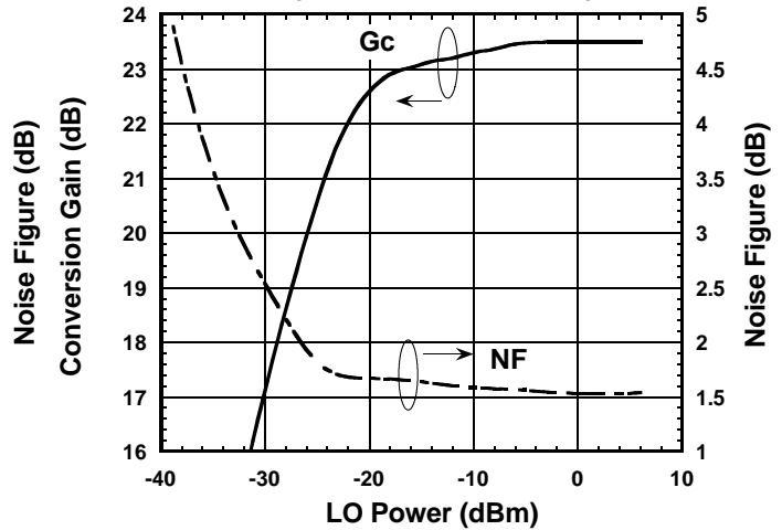
Conversion Gain , Noise Figure vs. LO Power
