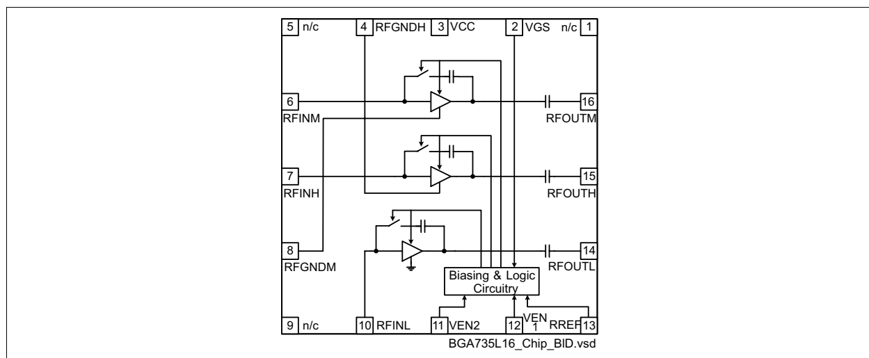
Figure 1 Block diagram of triple-band LNA
