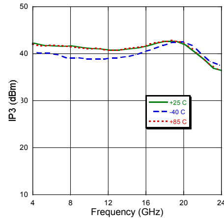
Output IP3
