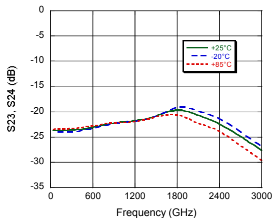
OUT-OUT Isolation to 3000 MHz OUT1-OUT2 & OUT1-OUT3
