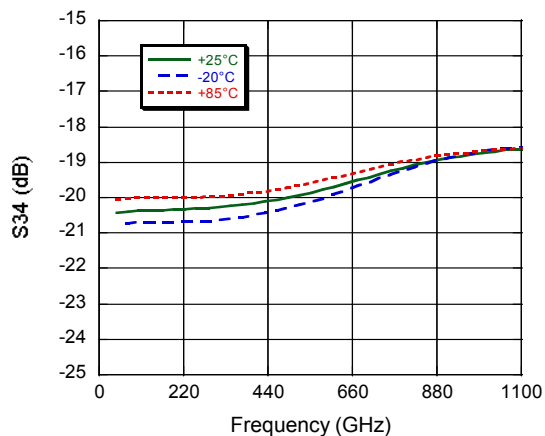
OUT-OUT Isolation to 1100 MHz OUT2-OUT3
