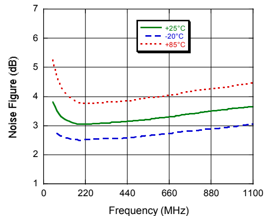
Noise Figure__OUT2 &amp; OUT3
