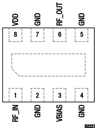
Figure 2. SKY65702-11 Pinout – 8-Pin MCM (Top View)
