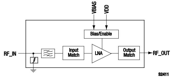
Figure 1. SKY65702-11 Block Diagram
