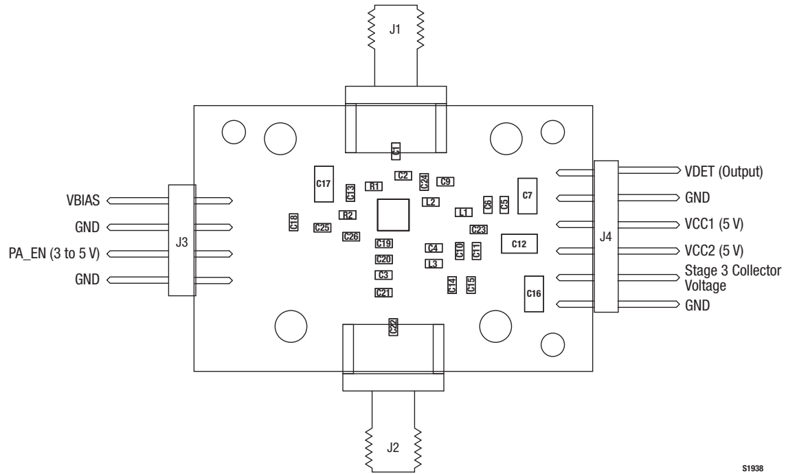
Figure 9. Evaluation Board Assembly Drawing
