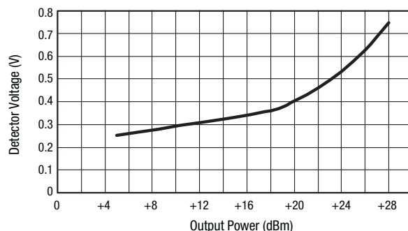
Figure 8. Detector Voltage vs Output Power
