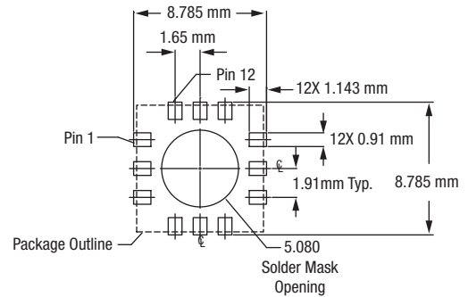
Solder Mask Opening Top View
