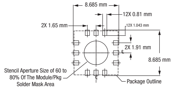
Stencil Aperture Top View
