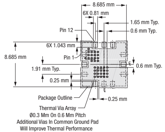
Metallization Top View
