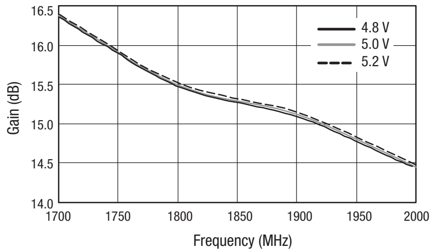
Figure 5. Gain vs Frequency Over VCC
