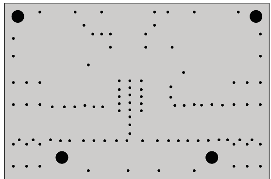
Layer 3: Ground
