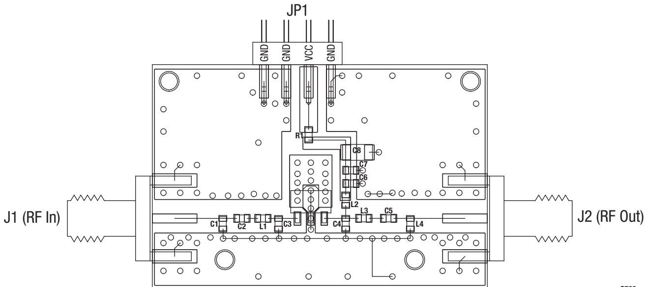
Figure 11. Evaluation Board Assembly Drawing
