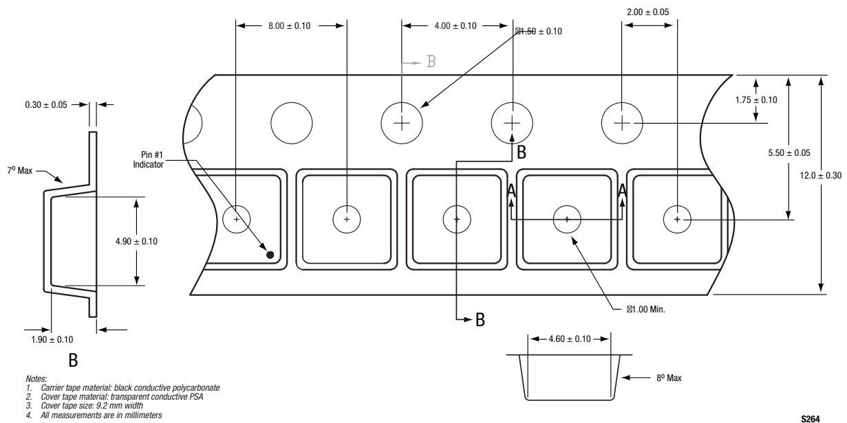
Figure 15. SKY65080-70LF Tape and Reel Dimensions
