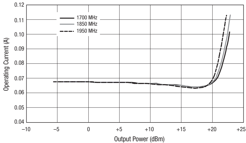
Figure 9. Operating Current vs Output Power Over Frequency
