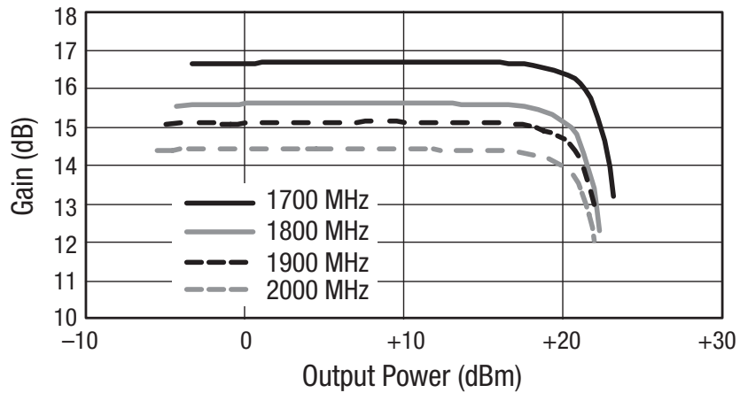
Figure 8. Gain vs Output Power Over Frequency
