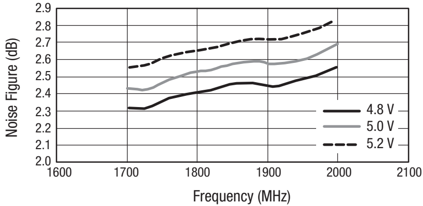
Figure 6. Noise Figure vs Frequency Over VCC
