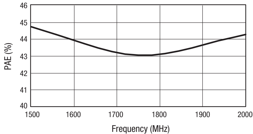
Figure 10. Power-Added Efficiency vs Frequency
