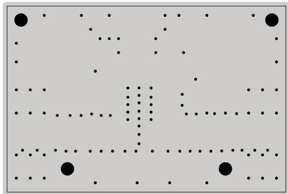
Layer 2: Ground
