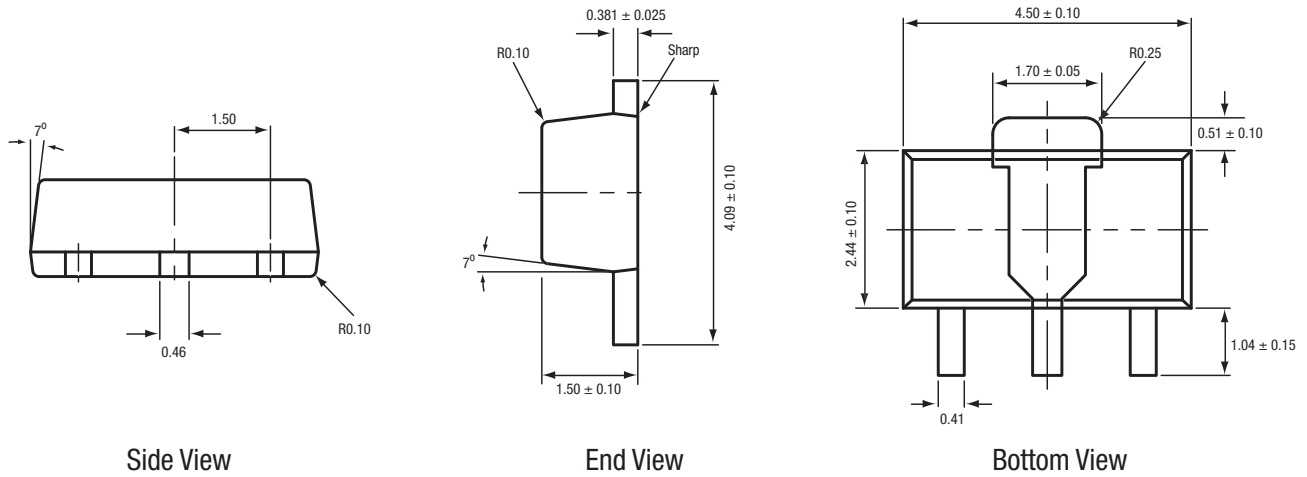
Figure 14. SKY65080-70LF (4-Pin SOT-89) Package Dimensions
