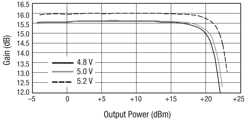
Figure 7. Typical Gain vs Output power Over VCC (CW @ 1800 MHz)
