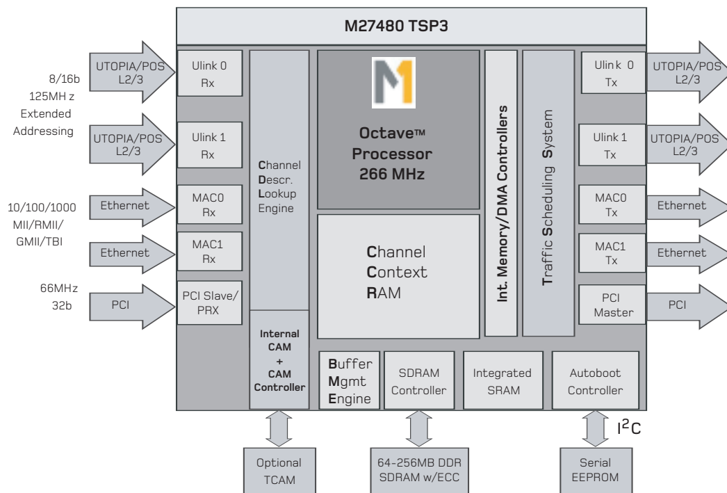
Figure 1: M27480 TSP3 Architecture
