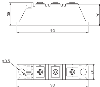
Fig. 8 - Outline Characteristics
