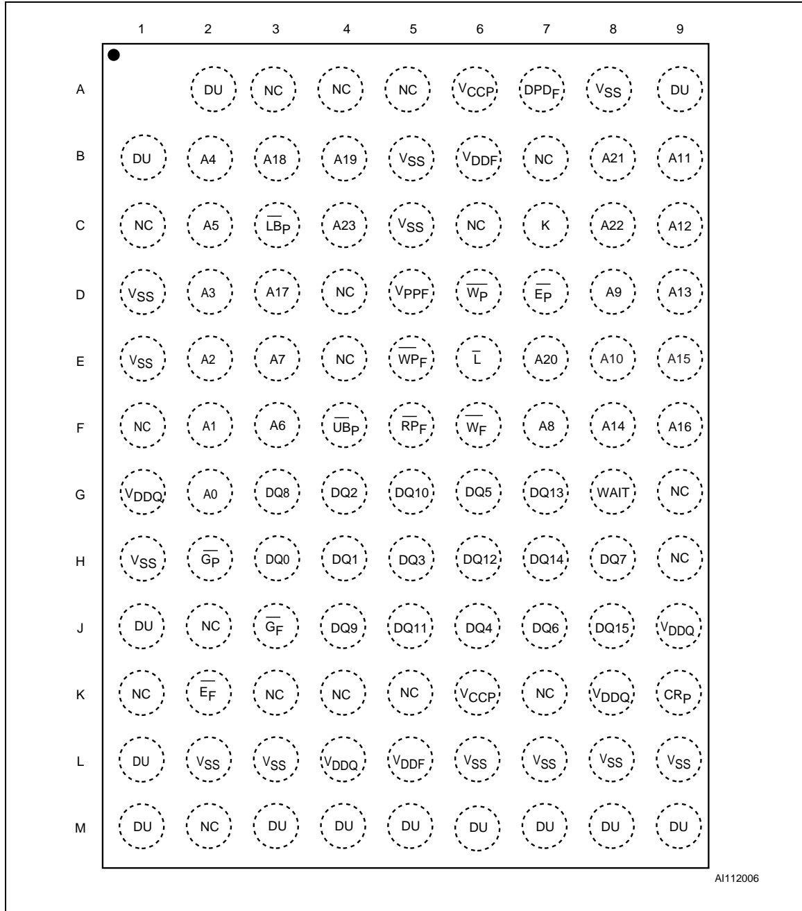
Figure 2. TFBGA connections (top view through package)
