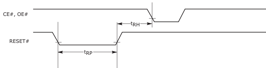
Figure 20. Reset Timings
