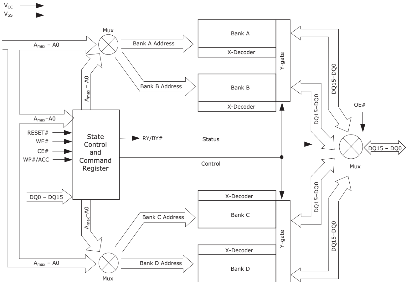
Figure 9.5 Simultaneous Operation Block Diagram for S29PL256N and S29PLI27N
