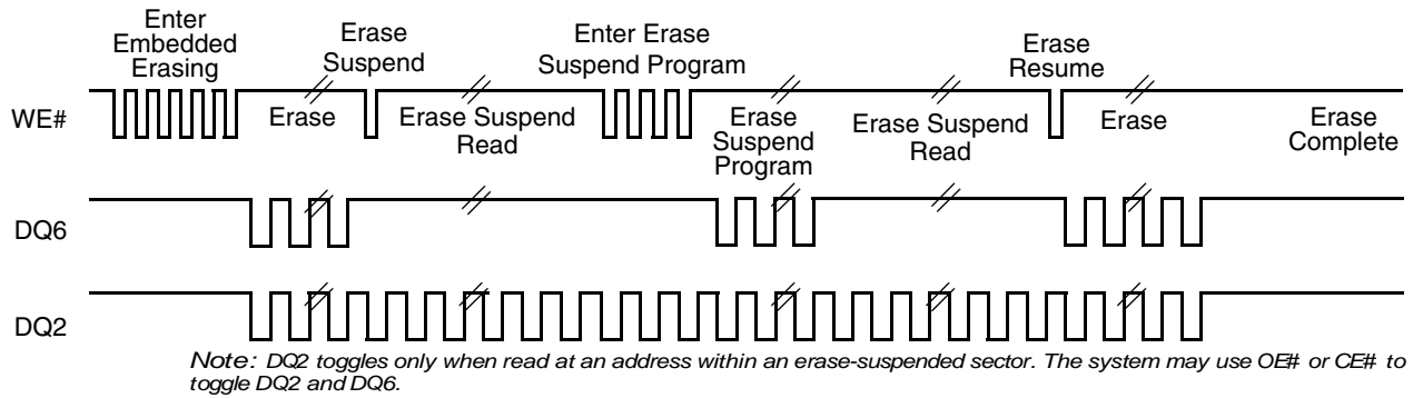
Figure I3.15 DQ2 vs. DQ6
