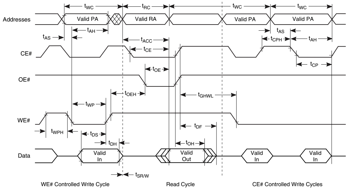
Figure I3.I2 Back-to-back Read/Write Cycle Timings
