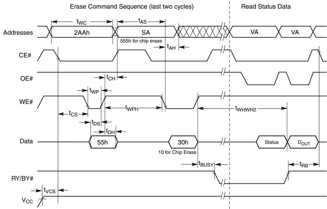
Figure I3.II Chip/Sector Erase Operation Timings
