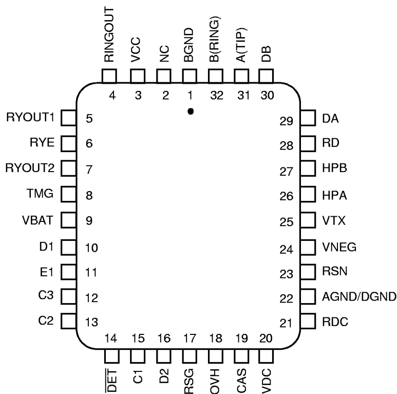
32-Pin PLCC
