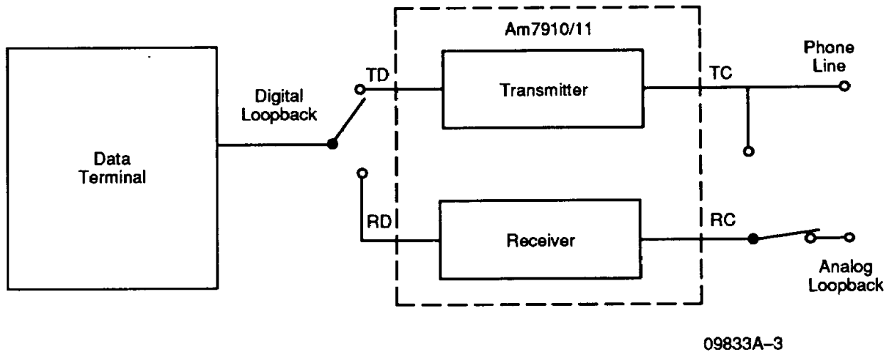
Figure 1. Analog Loopback
