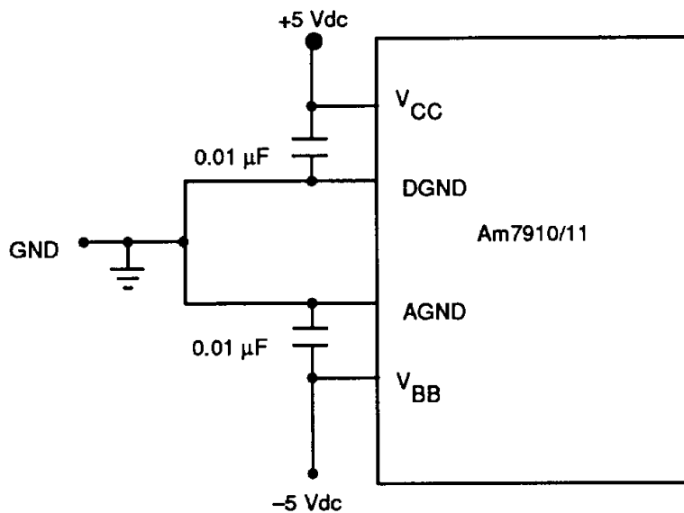
Figure 19. Power-Supply Connections
