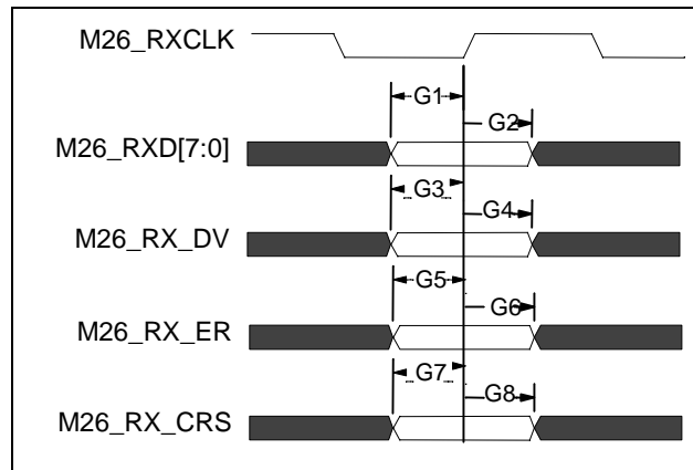
Figure 32 - AC Characteristics – Gigabit Media Independent Interface
