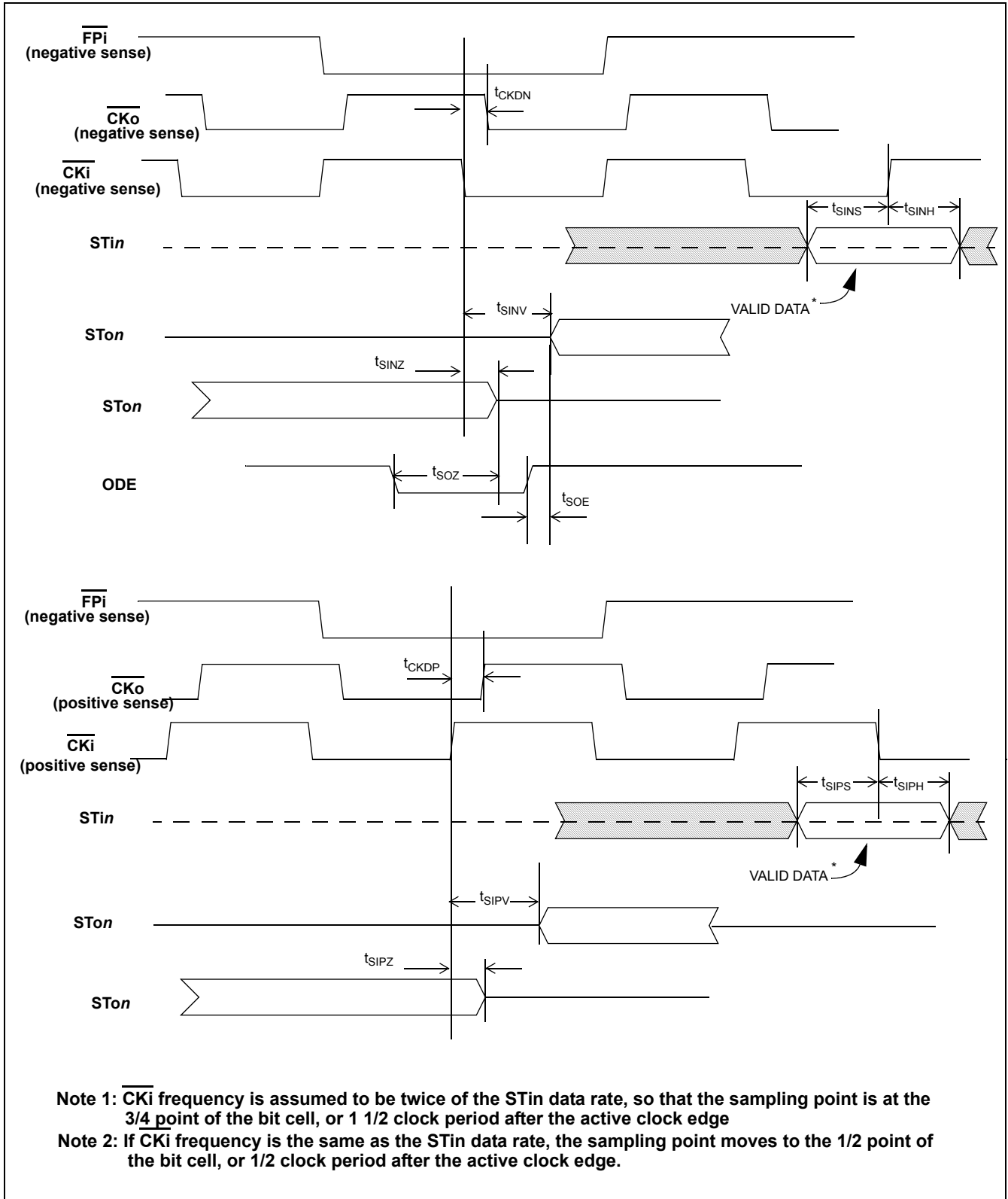
Figure 16 - Serial Data Timing to \overline{\text{CKi}}
