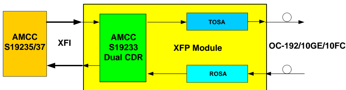
10 Gbps Line Card
