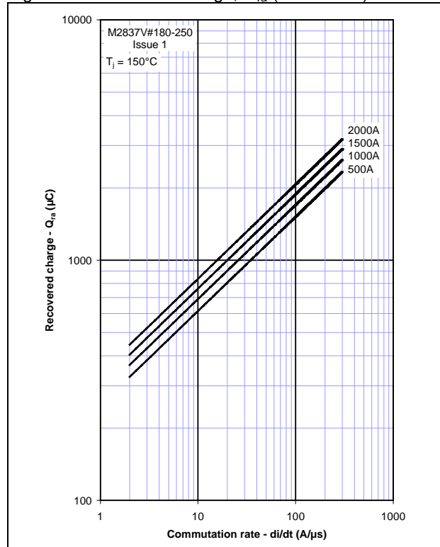
Figure 4 - Recovered charge, Q_{ra} (50% chord)
