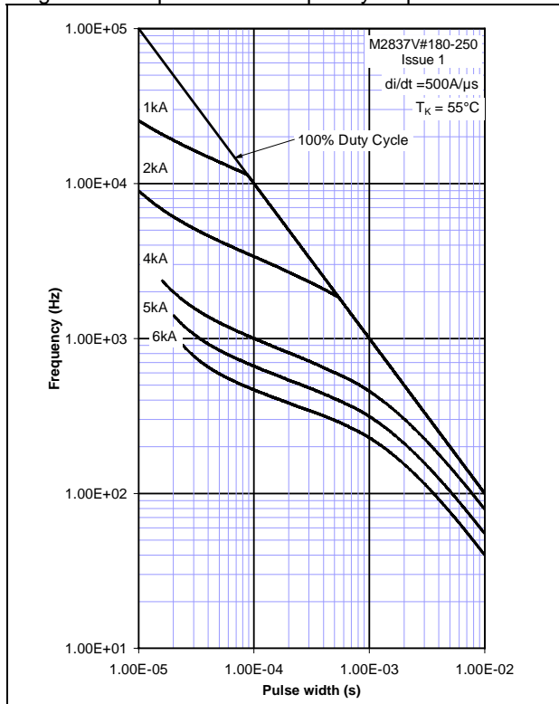
Figure 12 - Square wave frequency vs. pulse width
