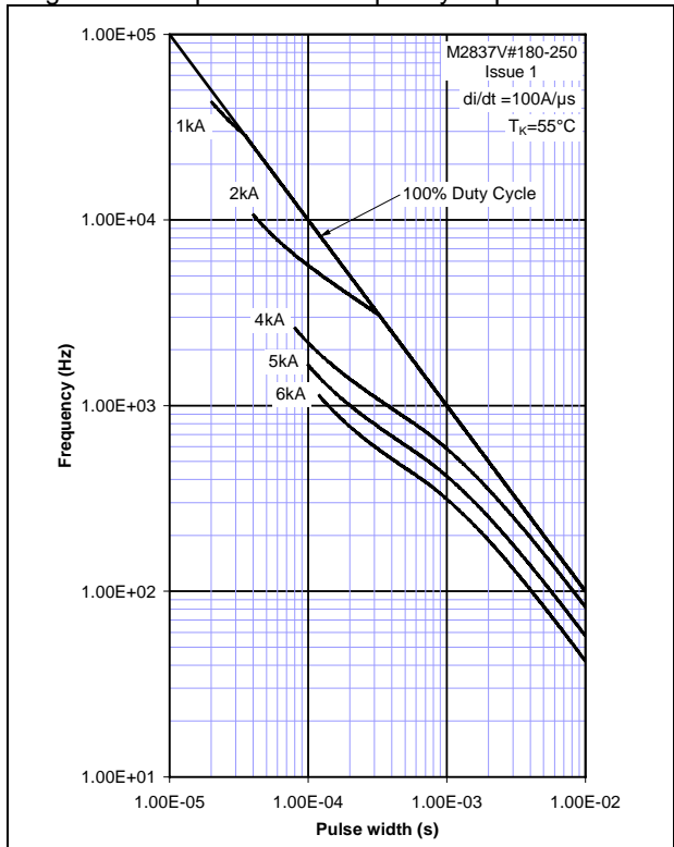
Figure 11 - Square wave frequency vs. pulse width
