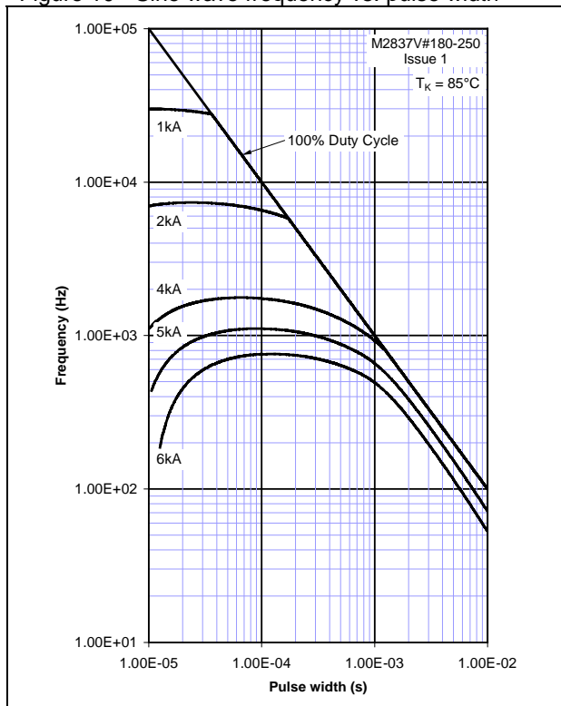
Figure 10 - Sine wave frequency vs. pulse width
