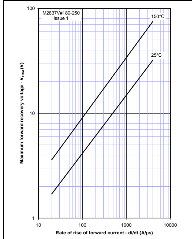
Figure 2 – Maximum forward recovery voltage
