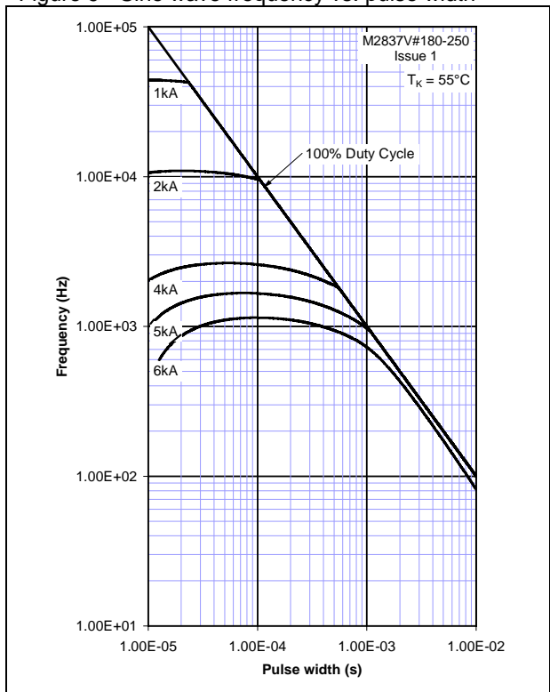
Figure 9 - Sine wave frequency vs. pulse width
