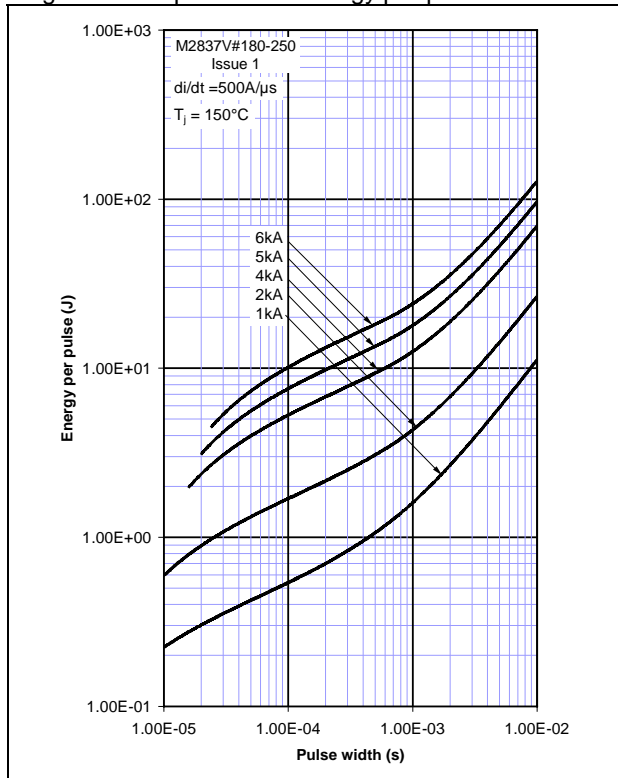
Figure 16 - Square wave energy per pulse
