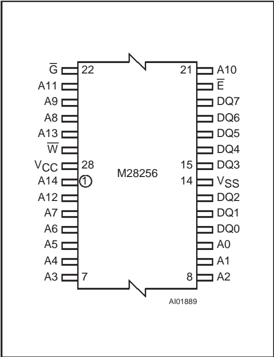
Figure 2D. TSOP Pin Connections
