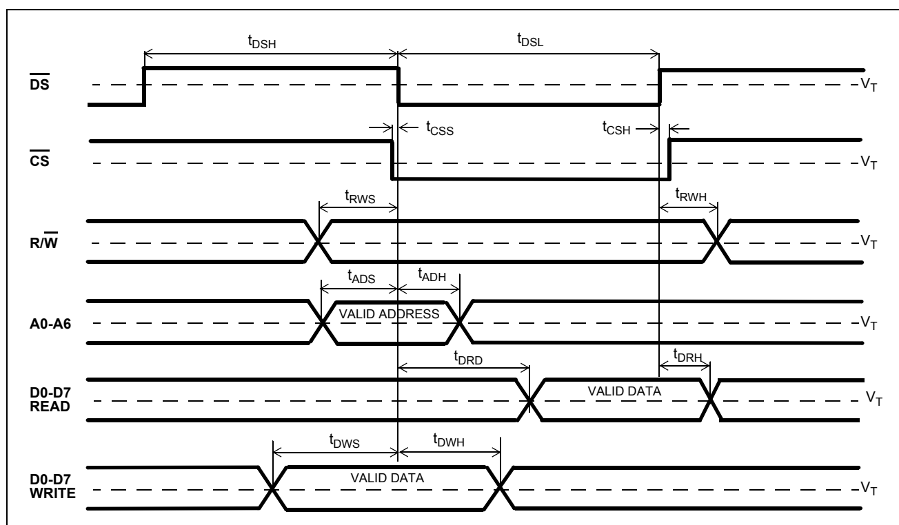
Figure 17 - Microport Timing
