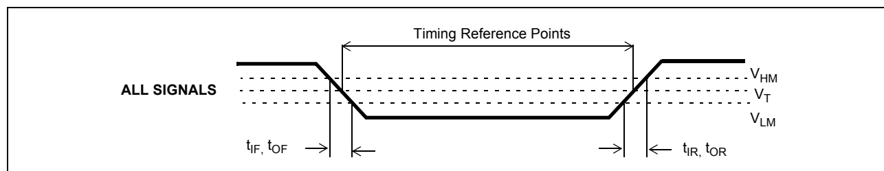
Figure 16 - Timing Parameters Measurement Voltage Levels
