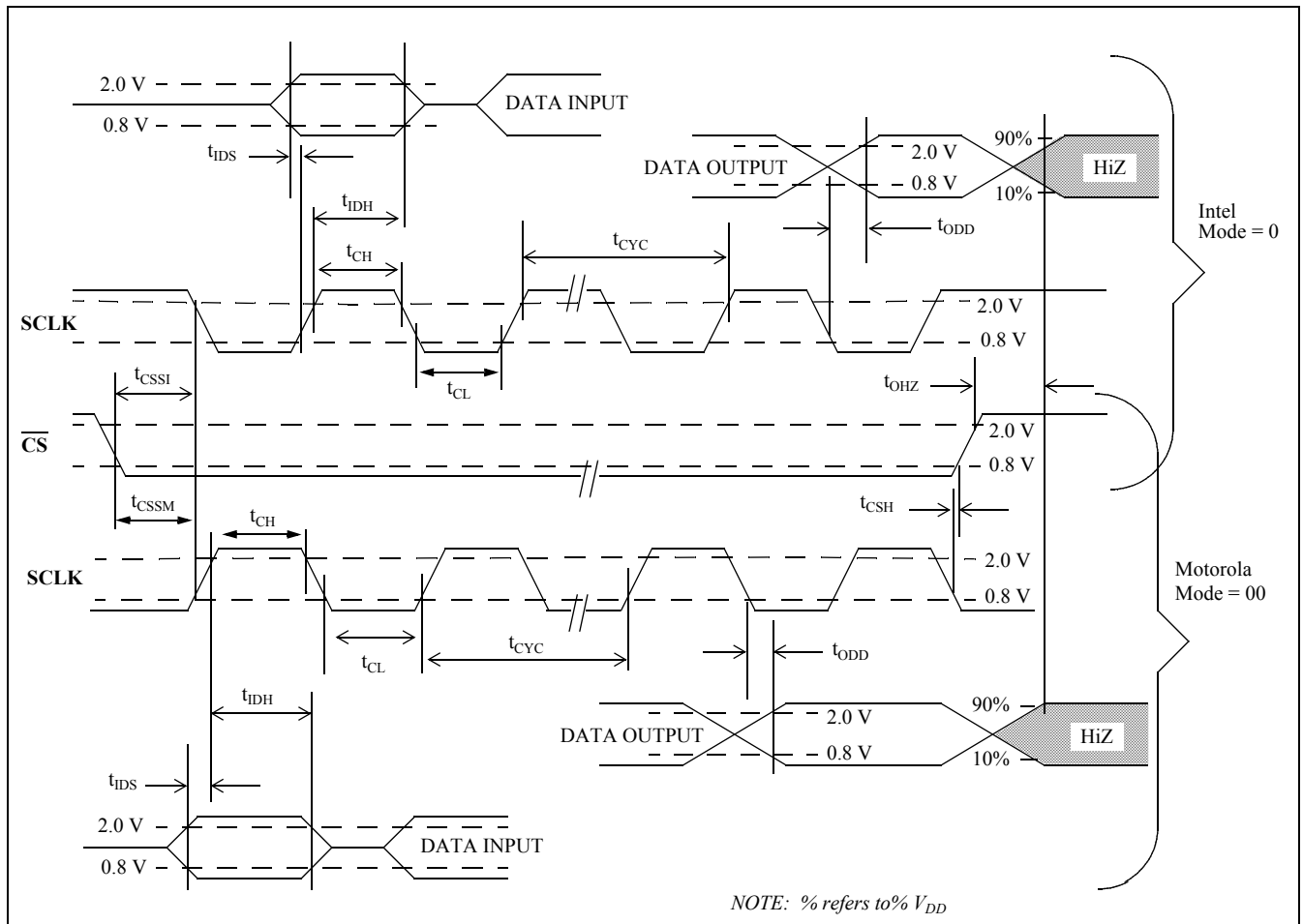
Figure 14 - Microport Timing
