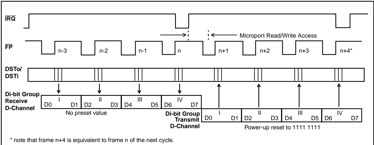
Figure 7a - D-Channel 16 kb/s Operation
