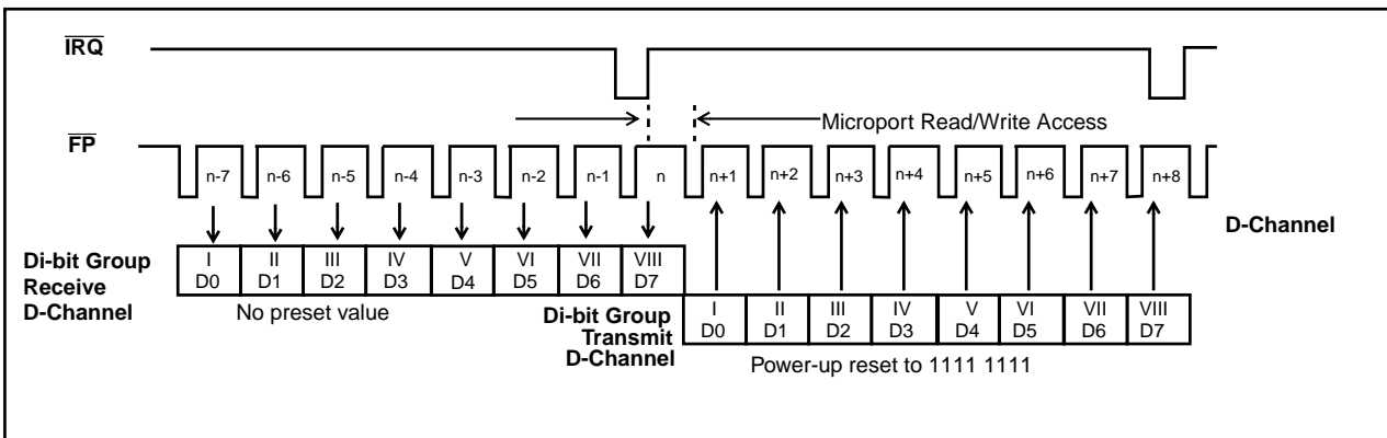
Figure 7c - D-Channel 8 kb/s Operation
