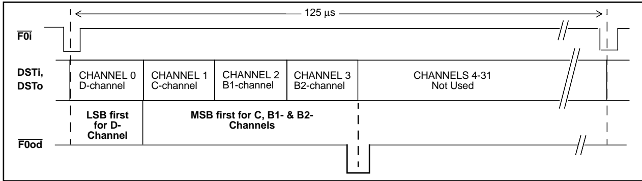
Figure 6 - ST-BUS Channel Assignment
