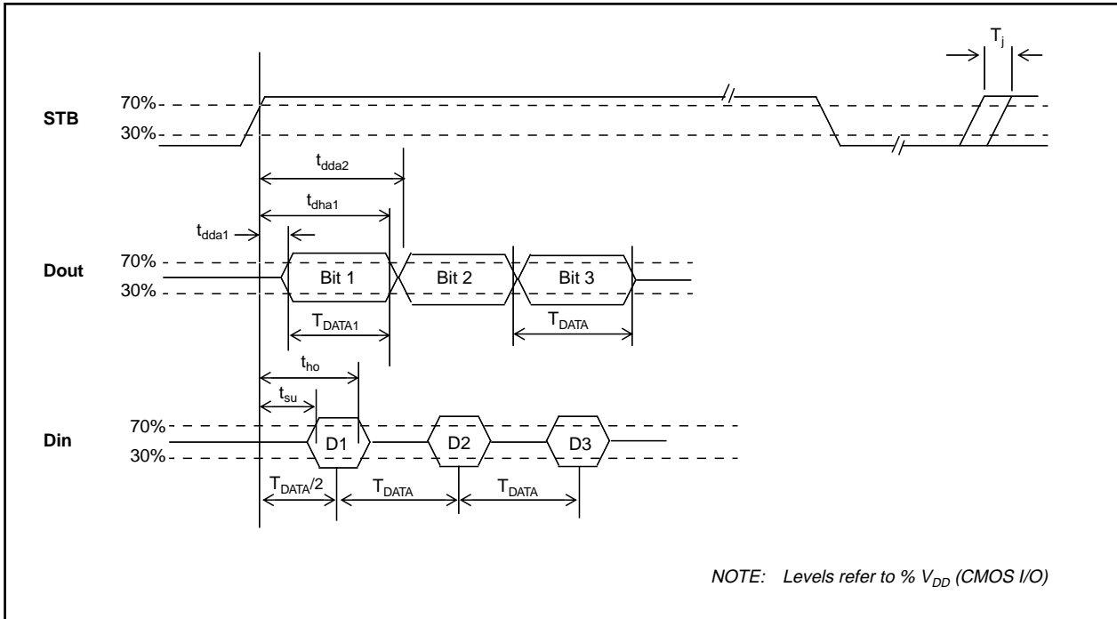
Figure 13 - SSI Asynchronous Timing Diagram
