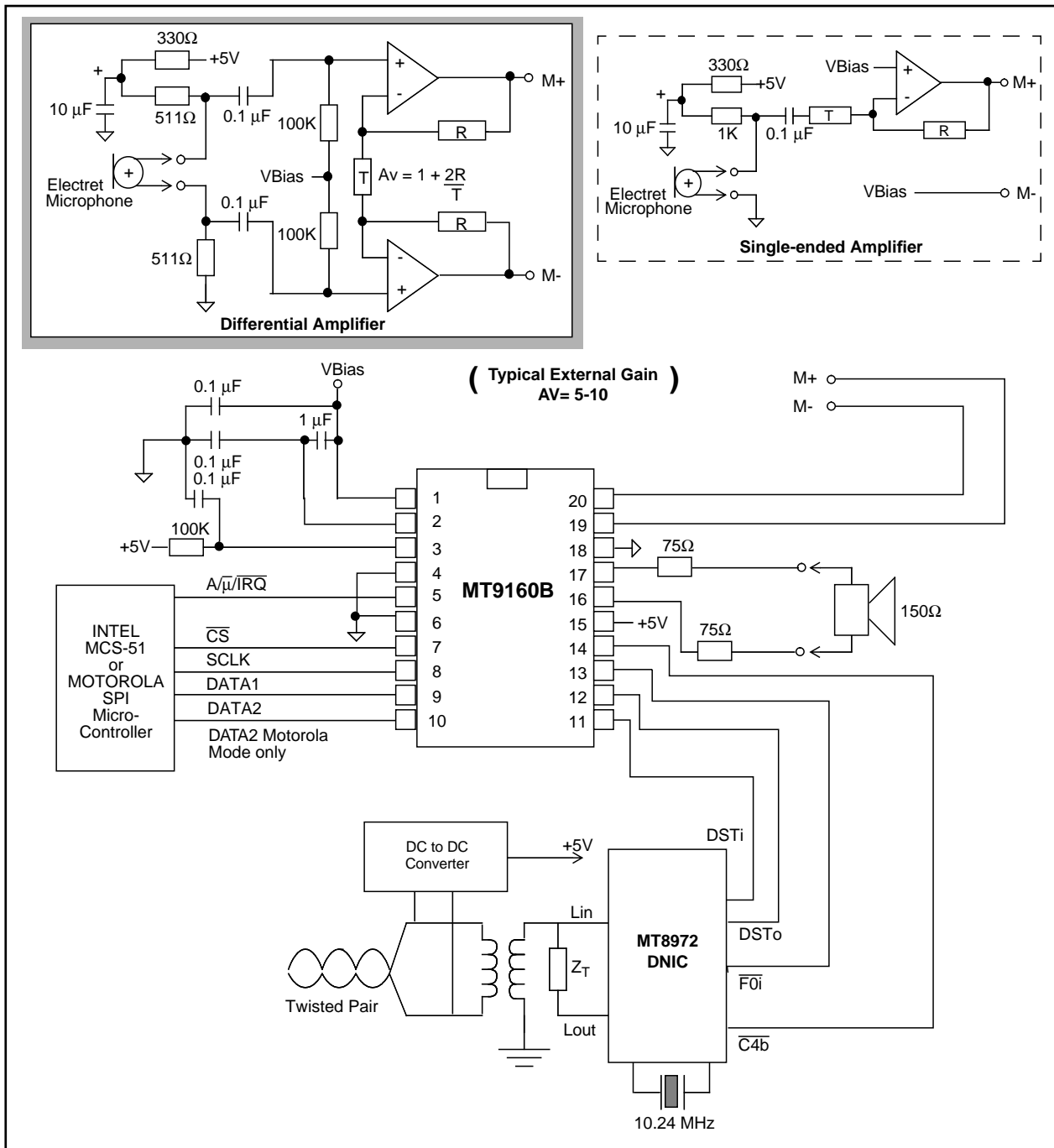
Figure 9 - Digital Telephone Set
