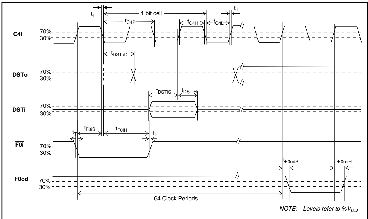
Figure 11 - ST-BUS Timing Diagram
