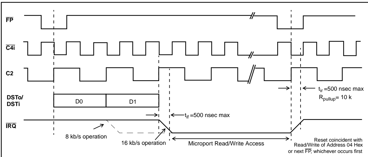
Figure 7b - \overline{\text{IRQ}} Timing Diagram
