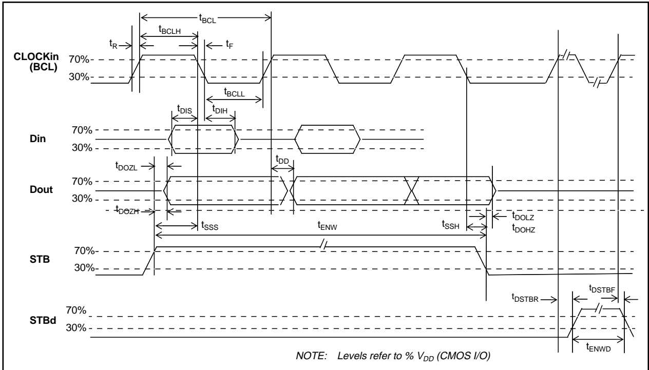
Figure 12 - SSI Synchronous Timing Diagram
