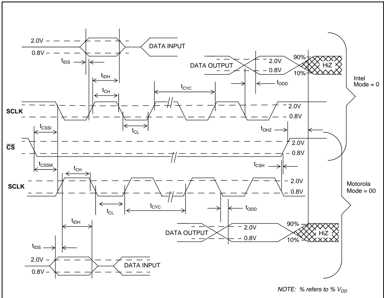
Figure 14 - Microport Timing
