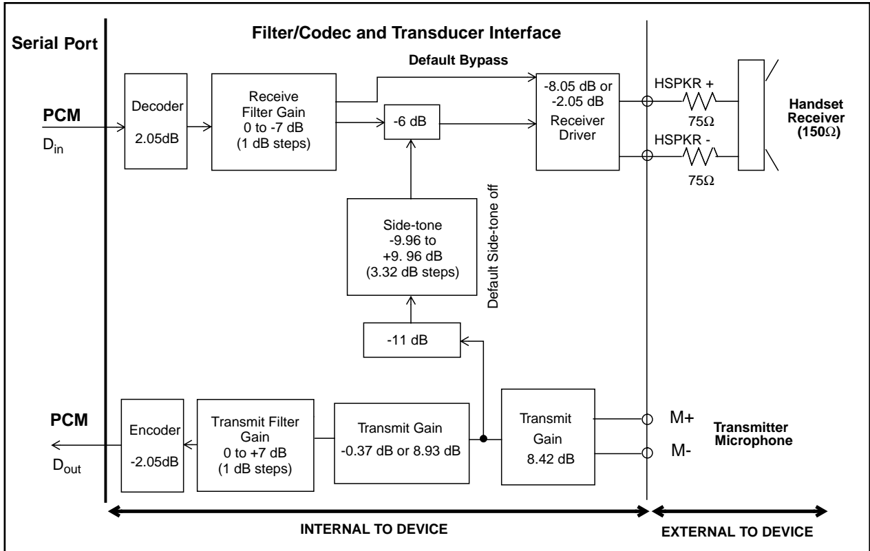
Figure 3 - Audio Gain Partitioning
