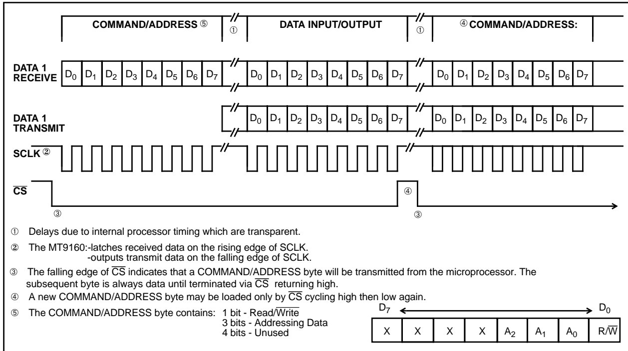
Figure 4 - Serial Port Relative Timing for Intel Mode 0
