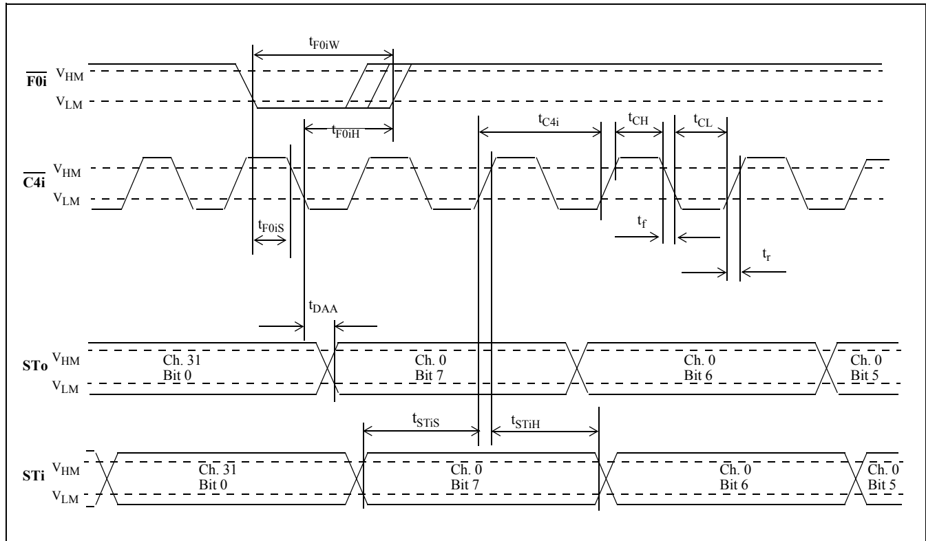
Figure 12 - ST-BUS Timing
