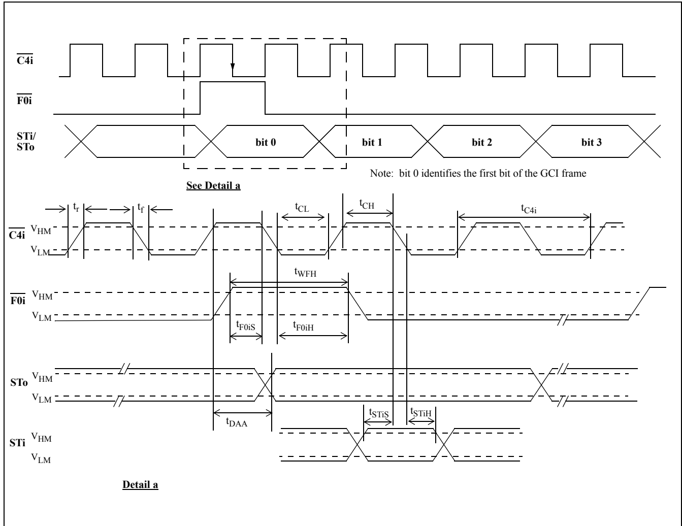
Figure 13 - GCI Timing
