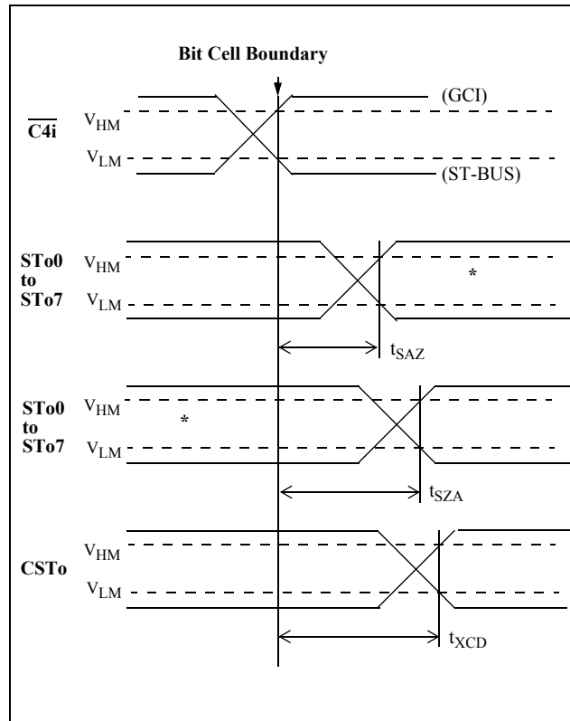
Figure 14 - Serial Outputs and External Control
