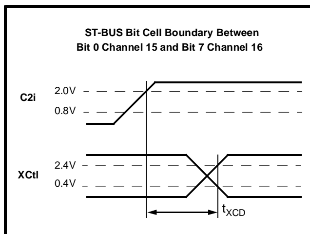
Figure 17 - XCtl Timing
