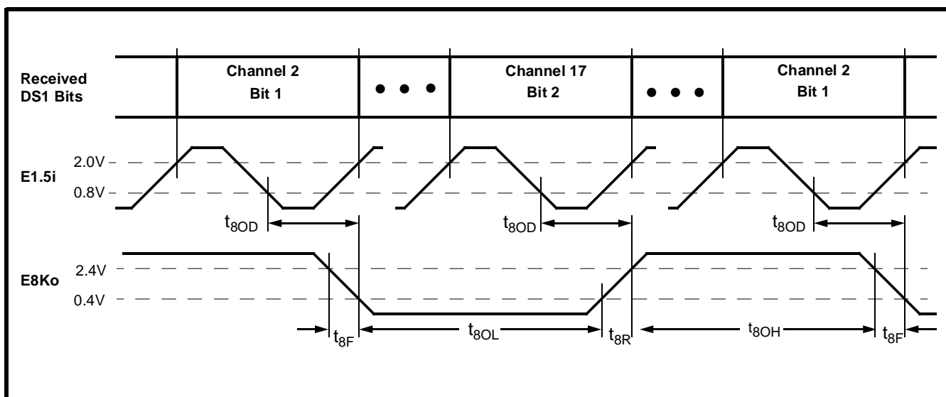
Figure 19 - E8Ko Timing
