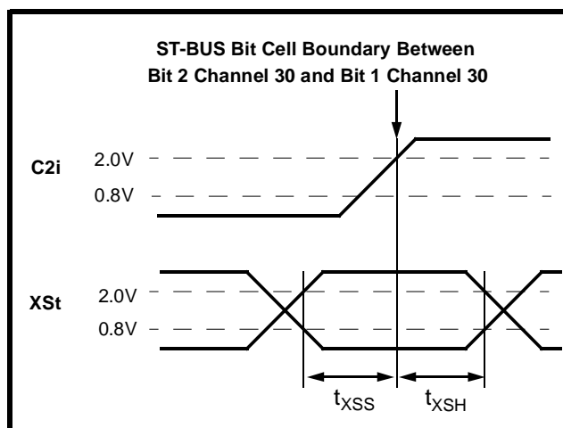
Figure 18 - XSt Timing
