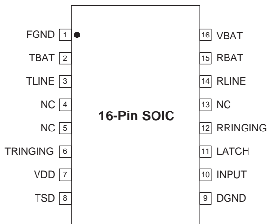
Figure 1. 16-Pin SOIC
