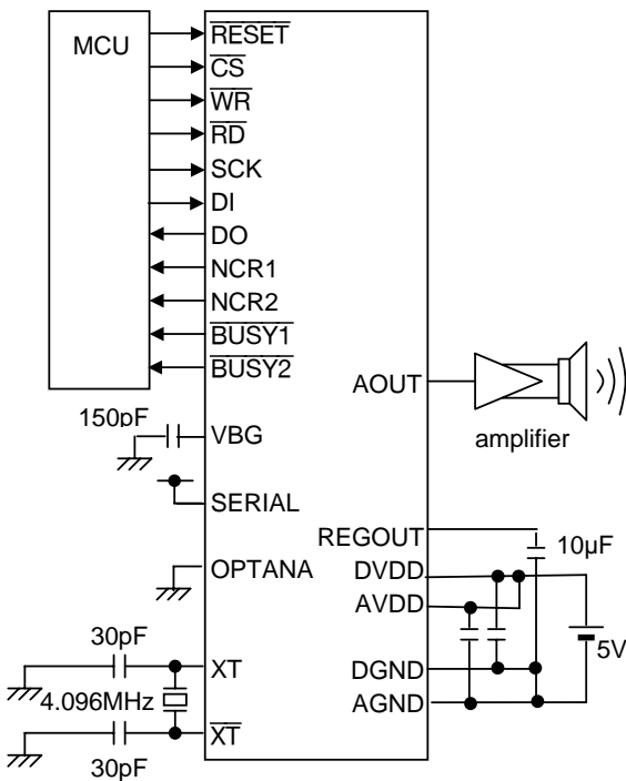
Serial Interface (at 5V)
