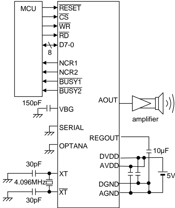
Parallel Interface (at 5V)
