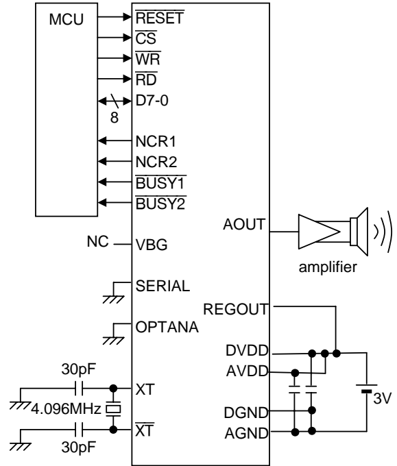
Parallel Interface(at 3V)
