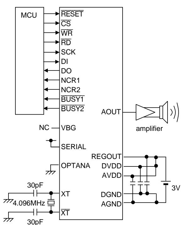
Serial Interface (at 3V)
