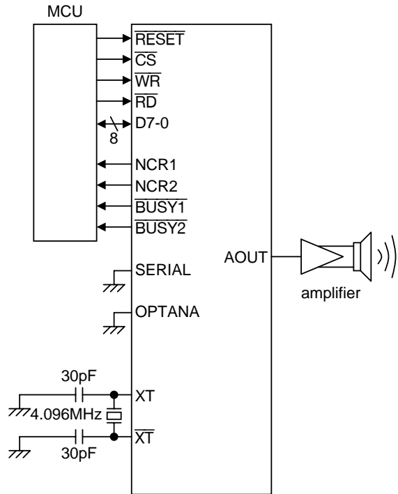
Parallel Interface
