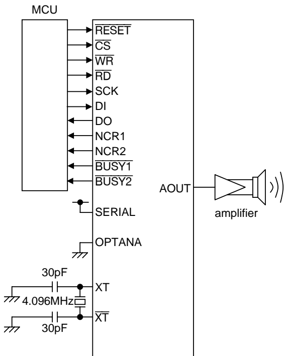
Serial Interface
