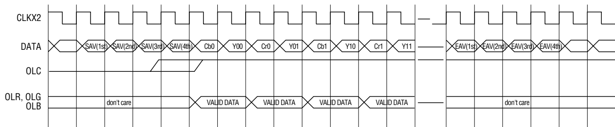
Overlay input timing (ITU-R BT.656 input mode)
