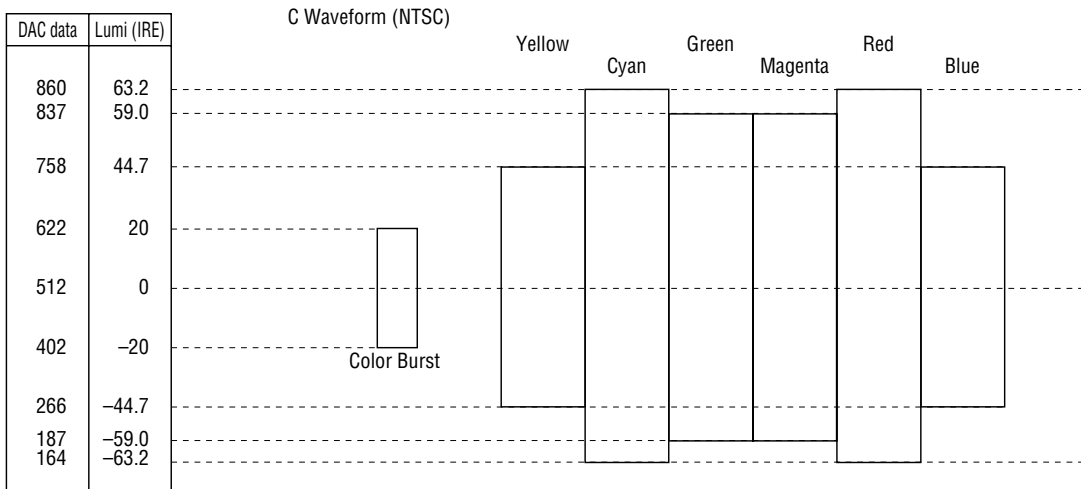
NTSC C Signal Output (Setup 0)
