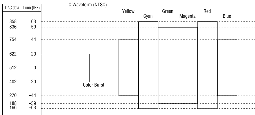
NTSC C Signal Output (Setup 7.5)
