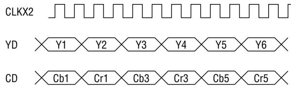
4:2:2 sampling at 8bit Y/8bit CbCr input
