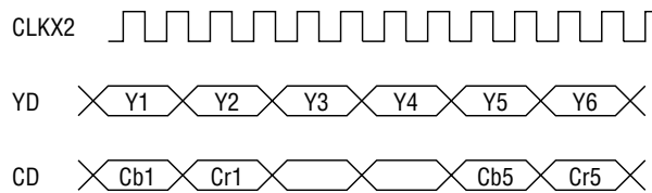
4:1:1 sampling at 8bit Y/8bit CbCr input
