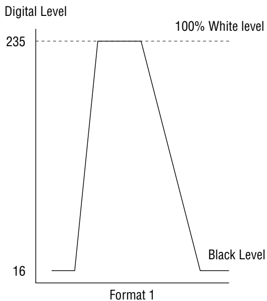
Input RGB signal level 1
