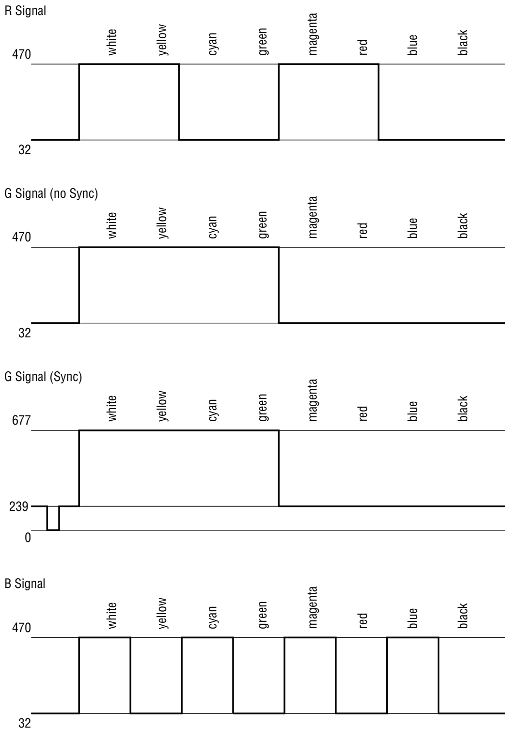
RGB Signal (Output Level Setting: 32-470)
