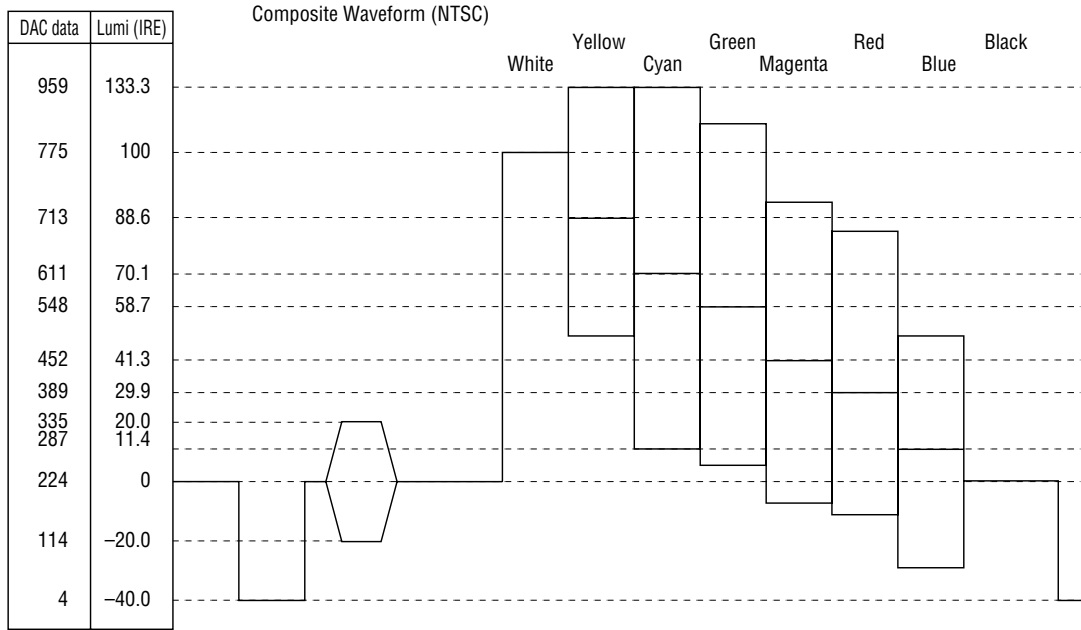
NTSC Composite Signal (Setup 0)
