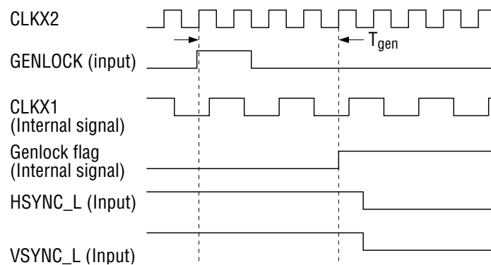
GENLOCK Input Timing
