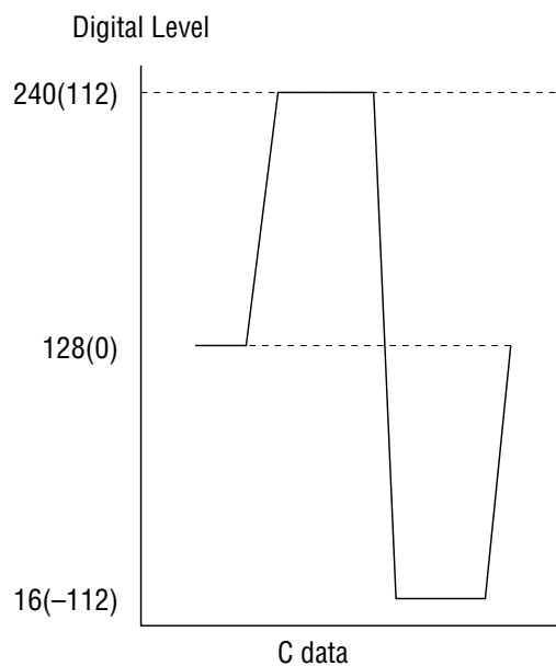
Input chrominance signal level
