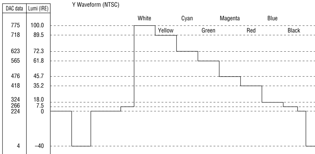
NTSC Y Signal Output (Setup 7.5)
