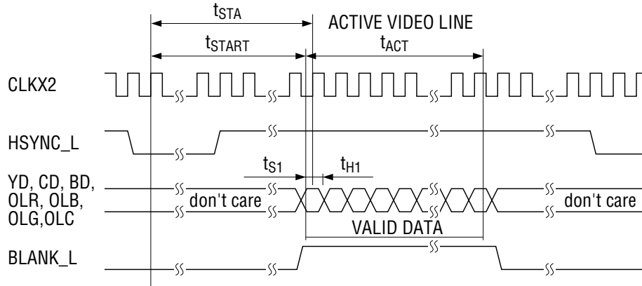
Video data input timing
