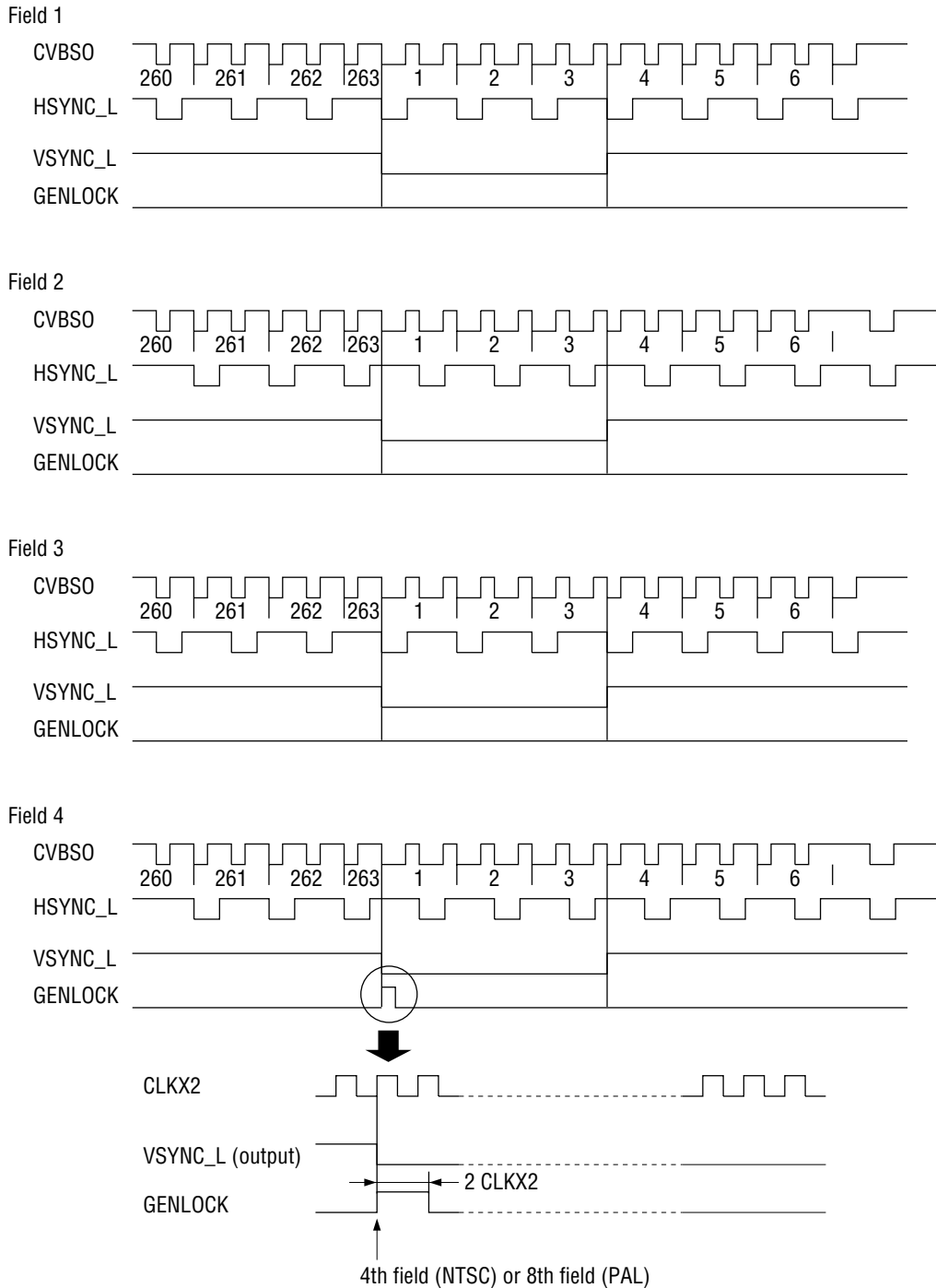
GENLOCK Output Timing
