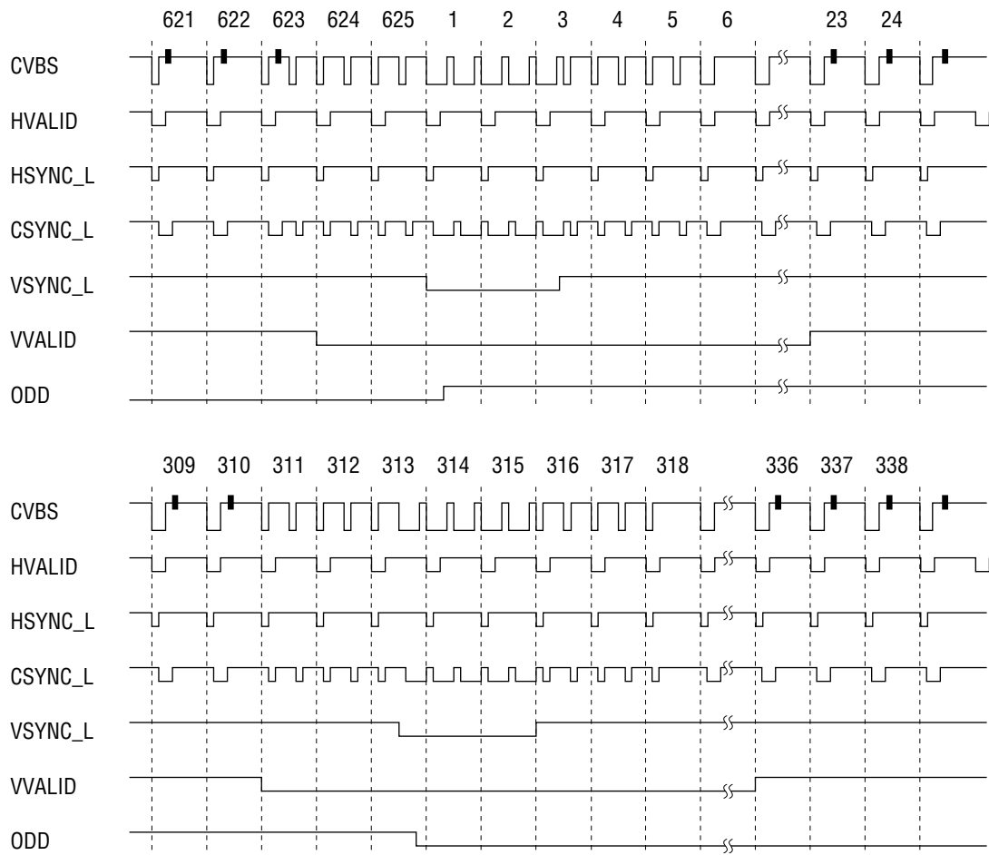
Vertical Synchronizing Signal (50 Hz)
