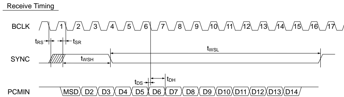
Figure 1 Basic Timing Diagram
