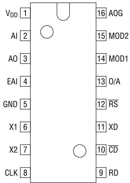
16-Pin Plastic DIP
