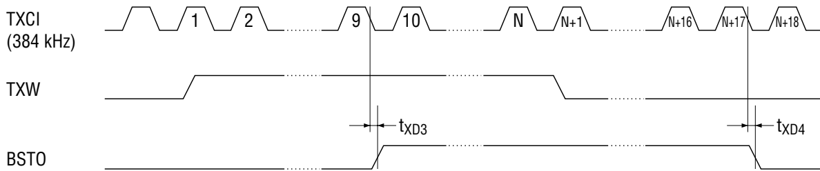
Figure 6 Transmit (Modulator) Digital Input/Output Timing
