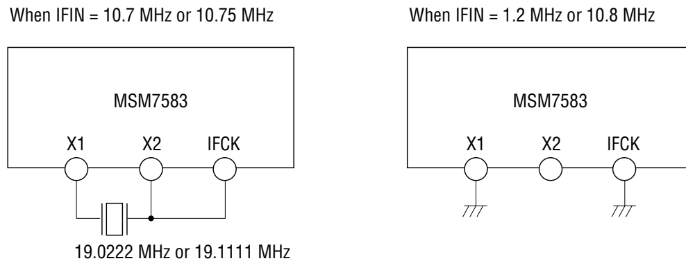
Figure 2 How to Use IFCK, X1, and X2
