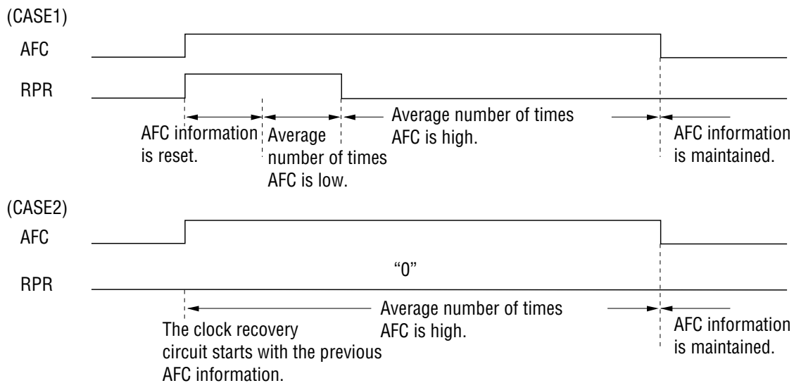
Figure 4 AFC Control Timing Diagram
