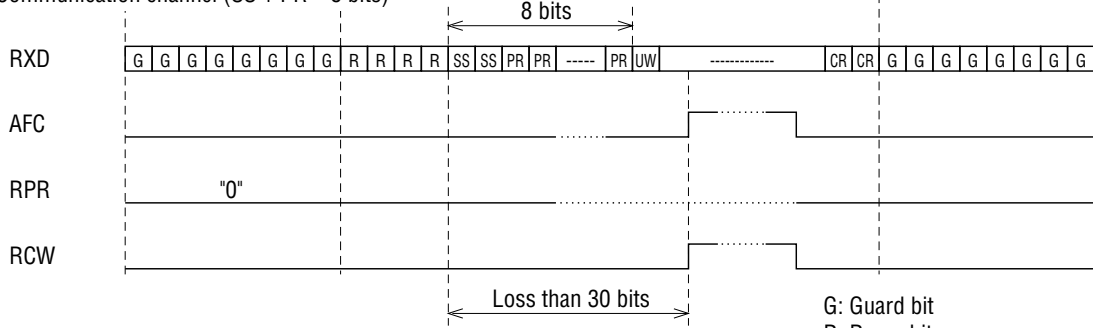
(2) Communication channel (SS + PR = 8 bits)
