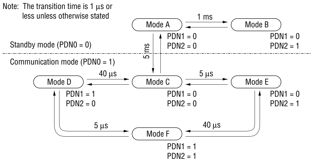
Figure 9 Power-Down State Transition Time
