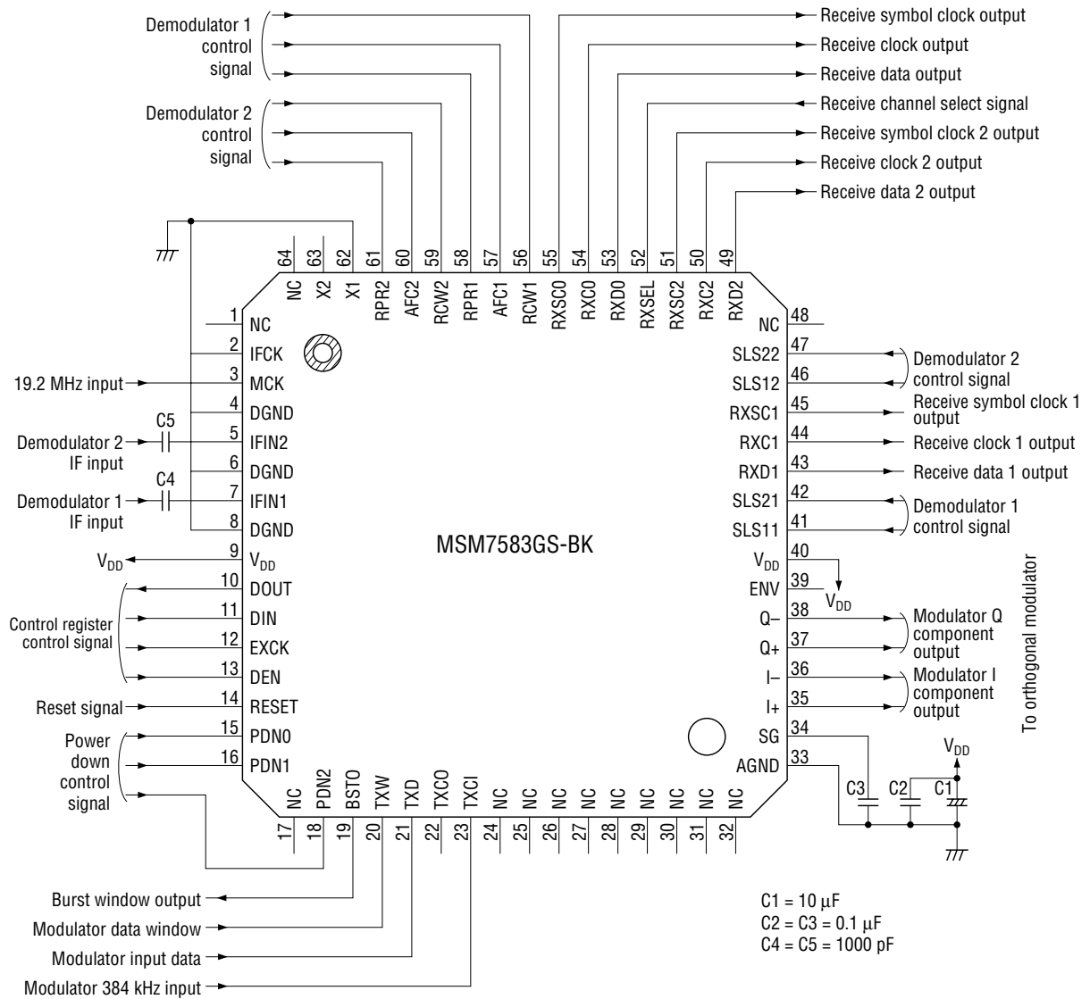
Figure 10 Example of Circuit Configuration
