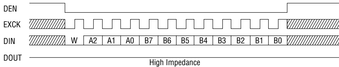
(a) Data Write Timing Diagram
