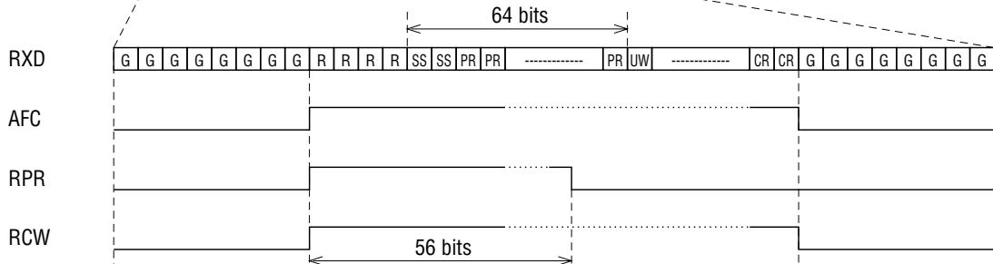
(1) Control channel/synchronous burst (SS + PR = 64 bits)
