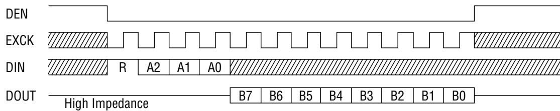
(b) Data Read Timing Diagram
