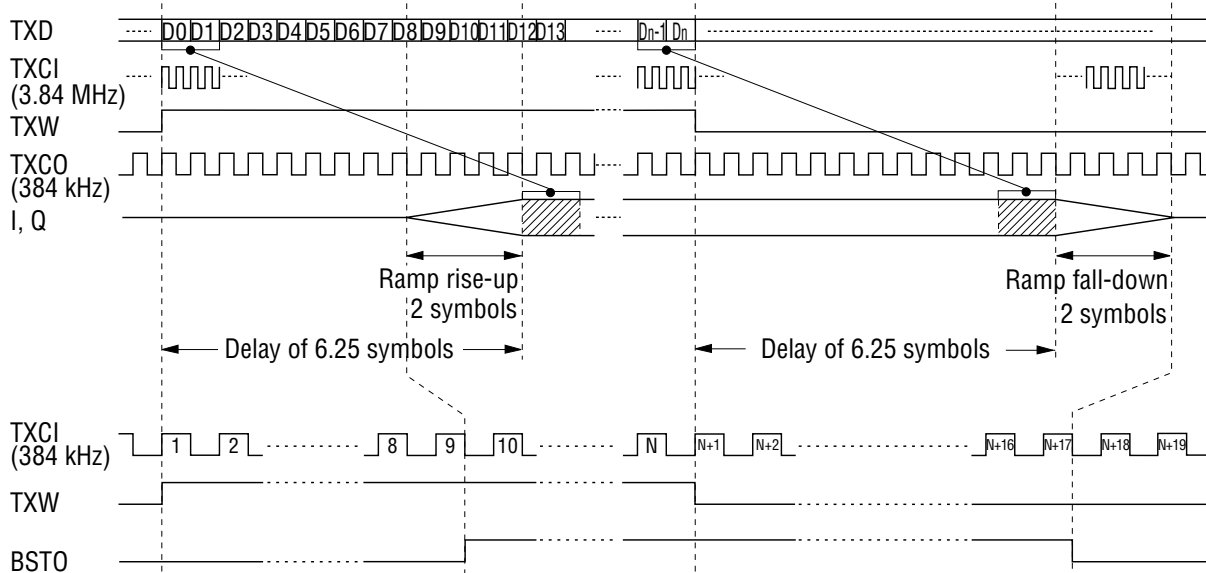
Figure 1 Transmitter Timing Diagram
