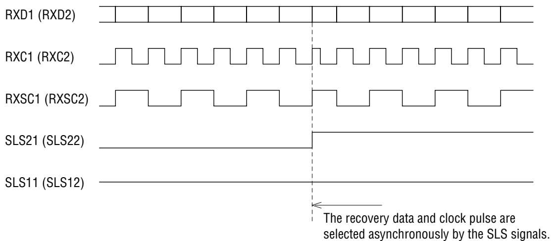
Figure 3 RXD, RXC, and RXSC Timing Diagram
