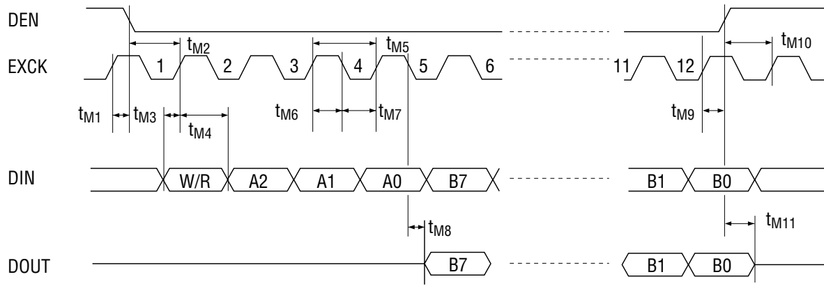
Figure 8 Serial Control Port Interface
