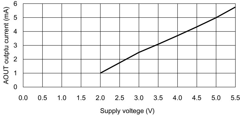
Relationship between supply voltage and AOUT output current (Ta = 20°C, VAOUT = V DD , PCM at maximum)
