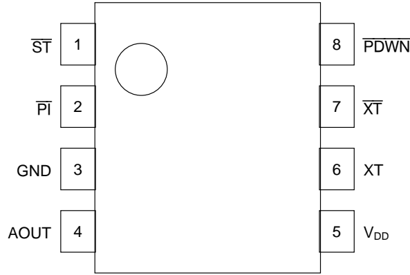
8-pin Plastic SOP
