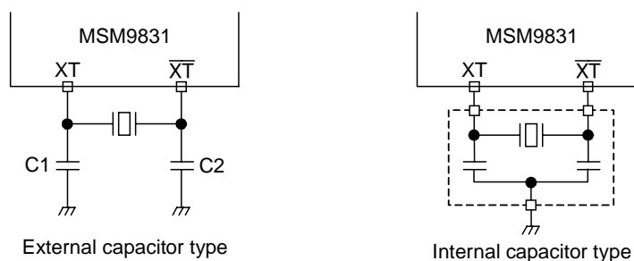
Figure 4 Oscillation Circuit with an external ceramic oscillator
