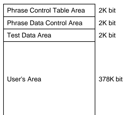
Figure 1 Memory Allocation of on-chip Mask ROM (384K bit)
