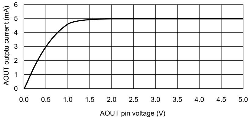
Relationship between AOUT pin voltage and AOUT output current (Ta = 25°C, V DD = 5.0 V, PCM at maximum)
