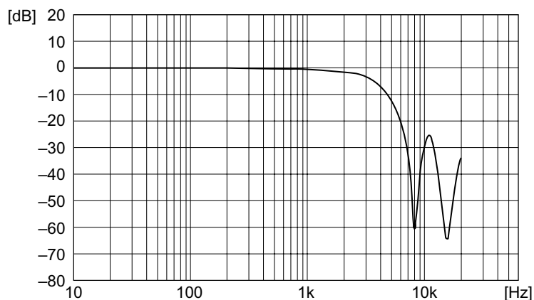
Figure 6 LPF Frequency Characteristics ( f_{SAM}=8 kHz)
