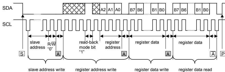
Figure 5 I 2 C Interface Read Timing: read-back mode
