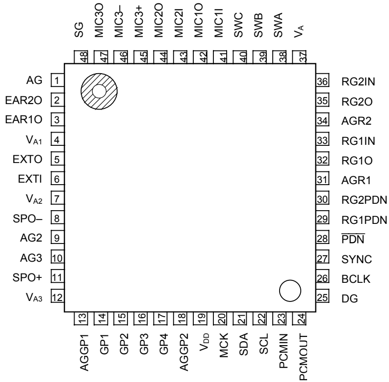
48-Pin Plastic TQFP
