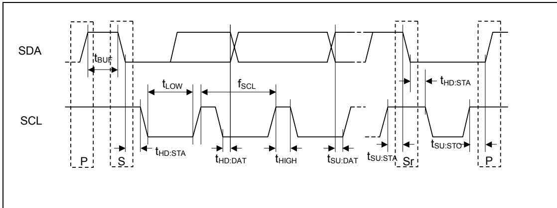
Figure 7 I 2 C Interface Timing
