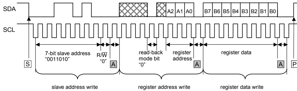
Figure 3 I 2 C Interface Write Timing
