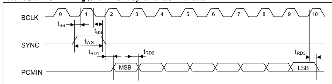
Figure 6 PCM Interface Timing
