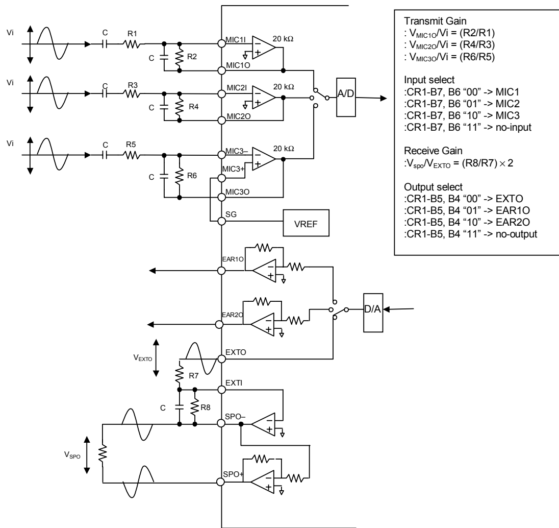
Figure 1 Analog Interface
