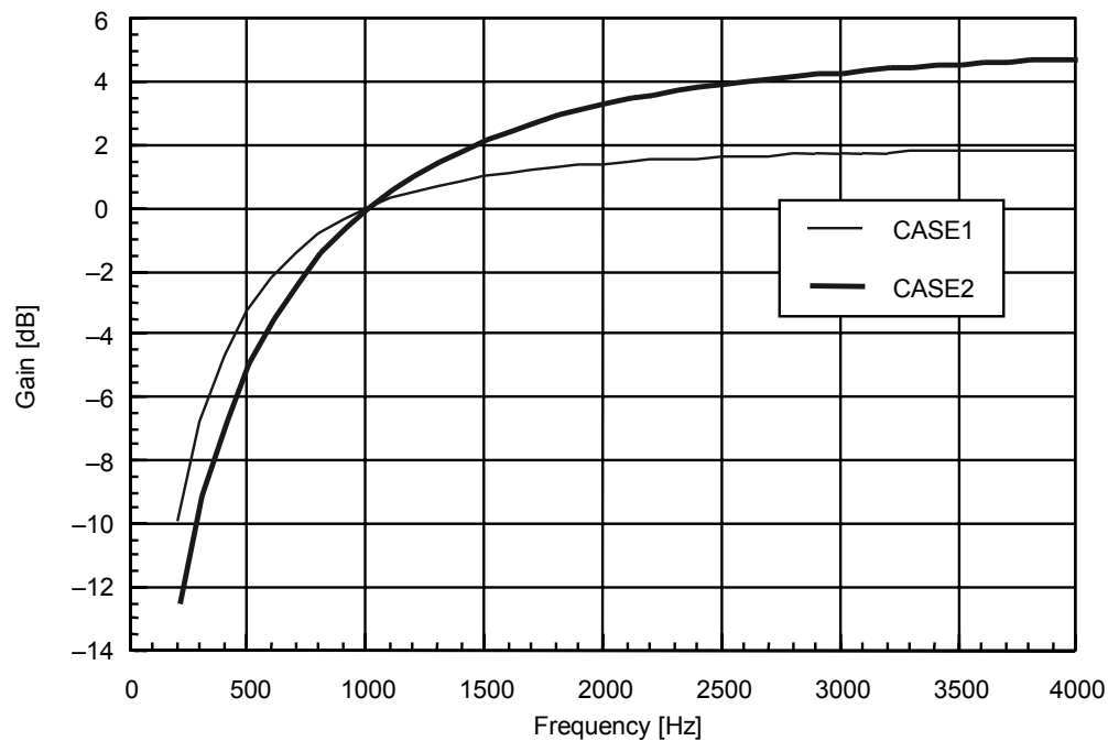
Figure 8 Slope Filter Frequency Characteristics
