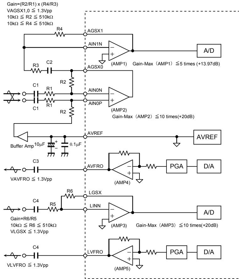
Figure 3 Analog Interface
